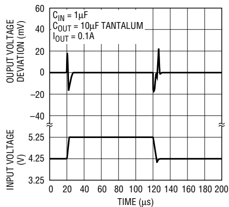
LT1117-2.8 Line Transient Response
