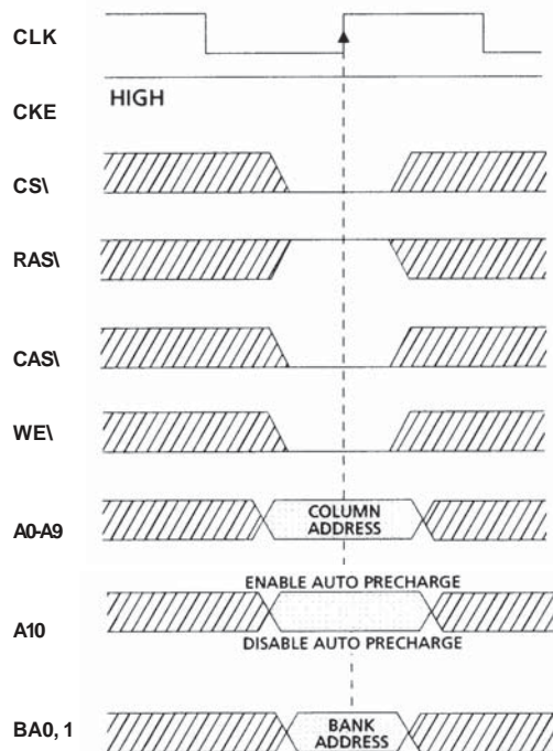
FIGURE 13: WRITE Command
