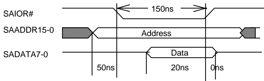
Waveform of IO Read Operation
