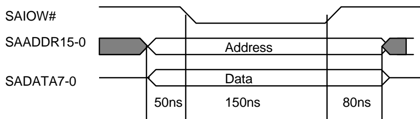
Waveform of IO Write Operation
