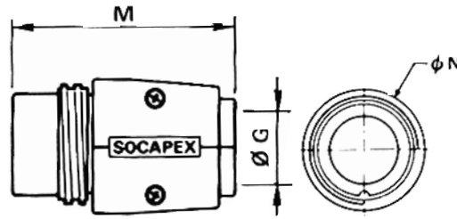
In-line female receptacle
