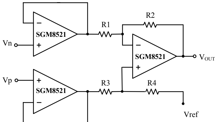
Figure 5. Instrumentation Amplifier
