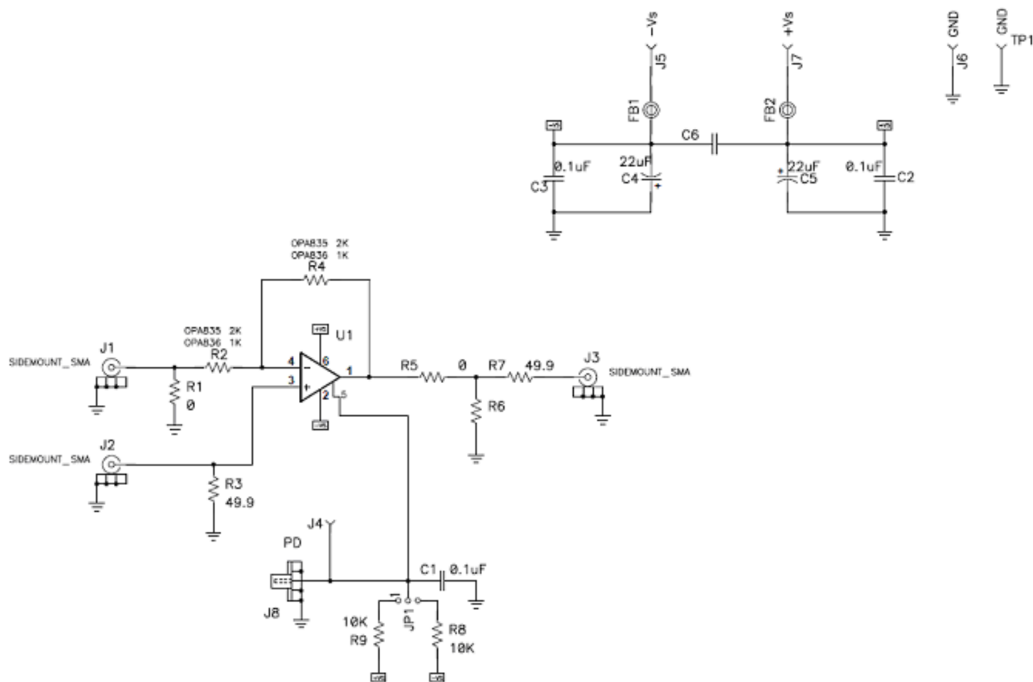
Figure 1. OPA835DBV and OPA836DBV EVM Schematic
