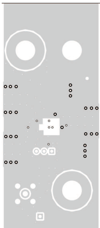
Figure 4. Ground Layer 3
