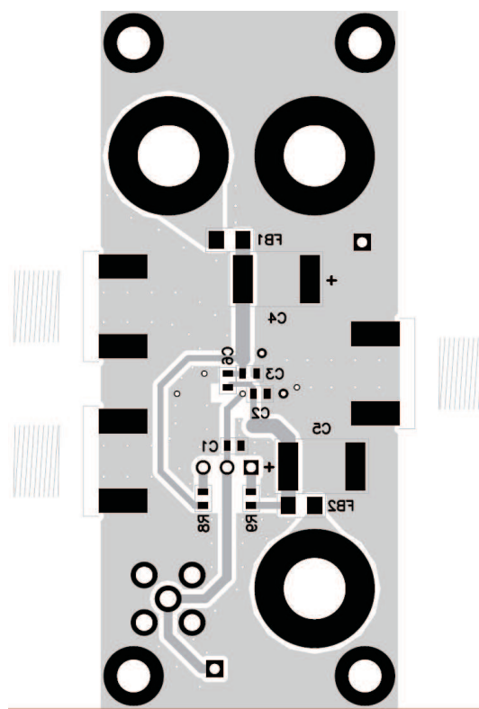
Figure 5. Bottom Layer
