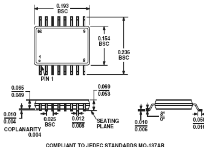
Figure 19. 16-Lead Shrink Small Outline Package [QSOP] (RQ-16)
