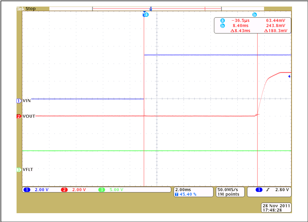
Figure 10. Startup, t_{\text{on}}
