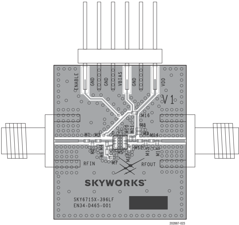
Figure 23. SKY67153-396LF Evaluation Board Assembly Diagram
