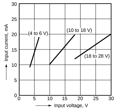
3. Input current vs. input voltage (10 A, 15 A, 20 A, 30 A, 40 A common)
