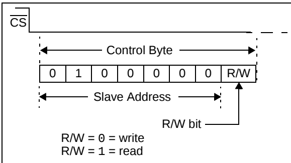
FIGURE 1-7: SPI CONTROL BYTE FORMAT
