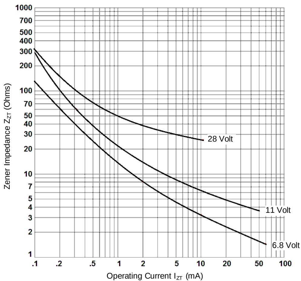
FIGURE 5 Zener Impedance vs. Operation Current (typical)
