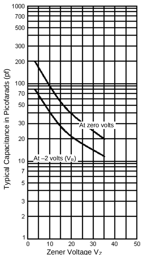
FIGURE 3 – Capacitance vs. Zener Voltage (typical)
