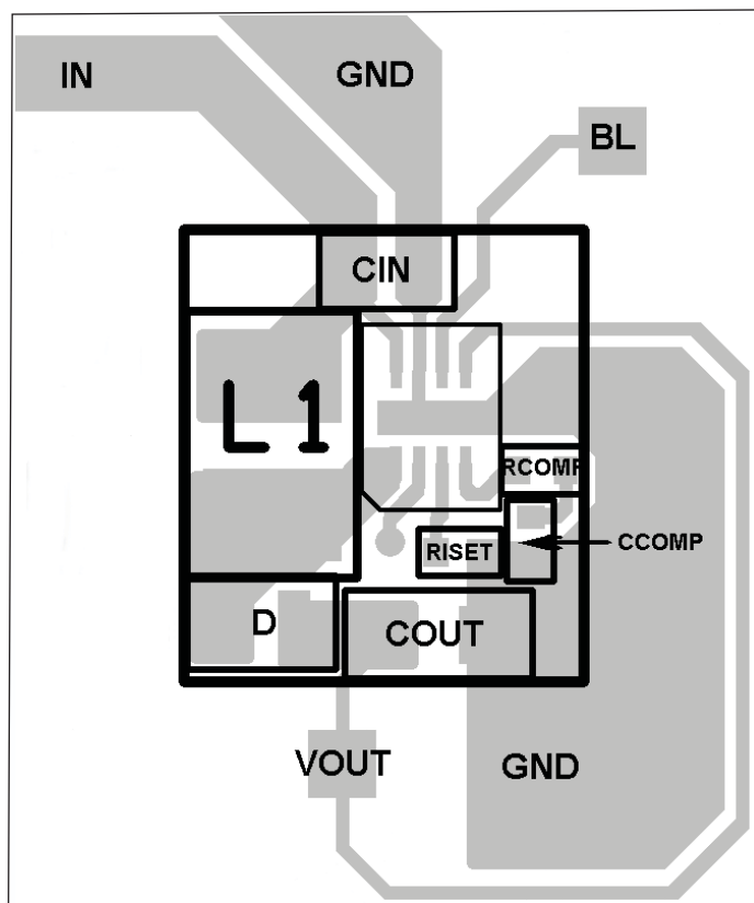
Figure 4– Layout
