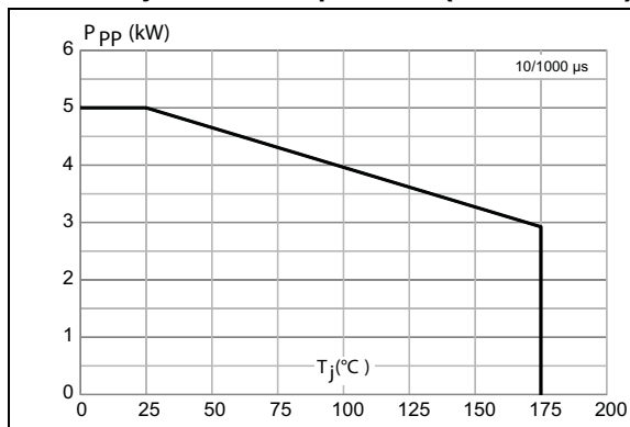
Figure 3. Peak pulse power dissipation versus initial junction temperature (LDP01-30AY)
