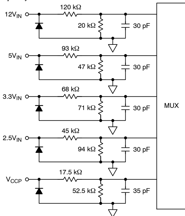
Figure 14. Internal Structure of Analog Inputs
