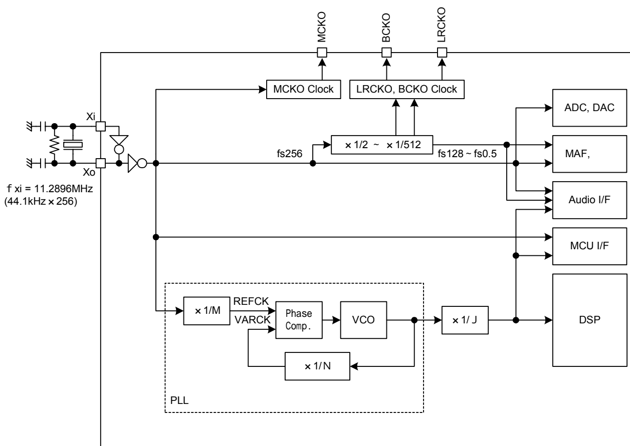
Figure 2 Block diagram of clock generator circuit
