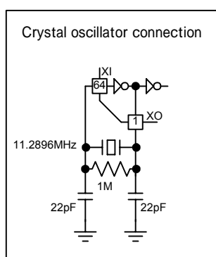
Figure 3 Example of oscillator circuit
