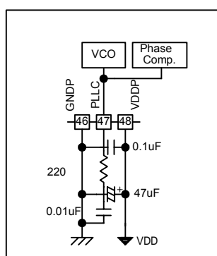
Figure 4 Example of PLL circuit
