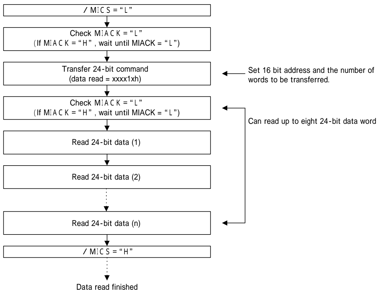
Figure 8 shows the 24-bit data read procedure.
