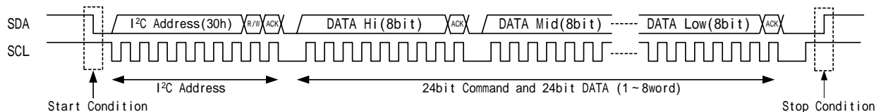
Figure 10 Data Transmission Format in I 2 C Mode
