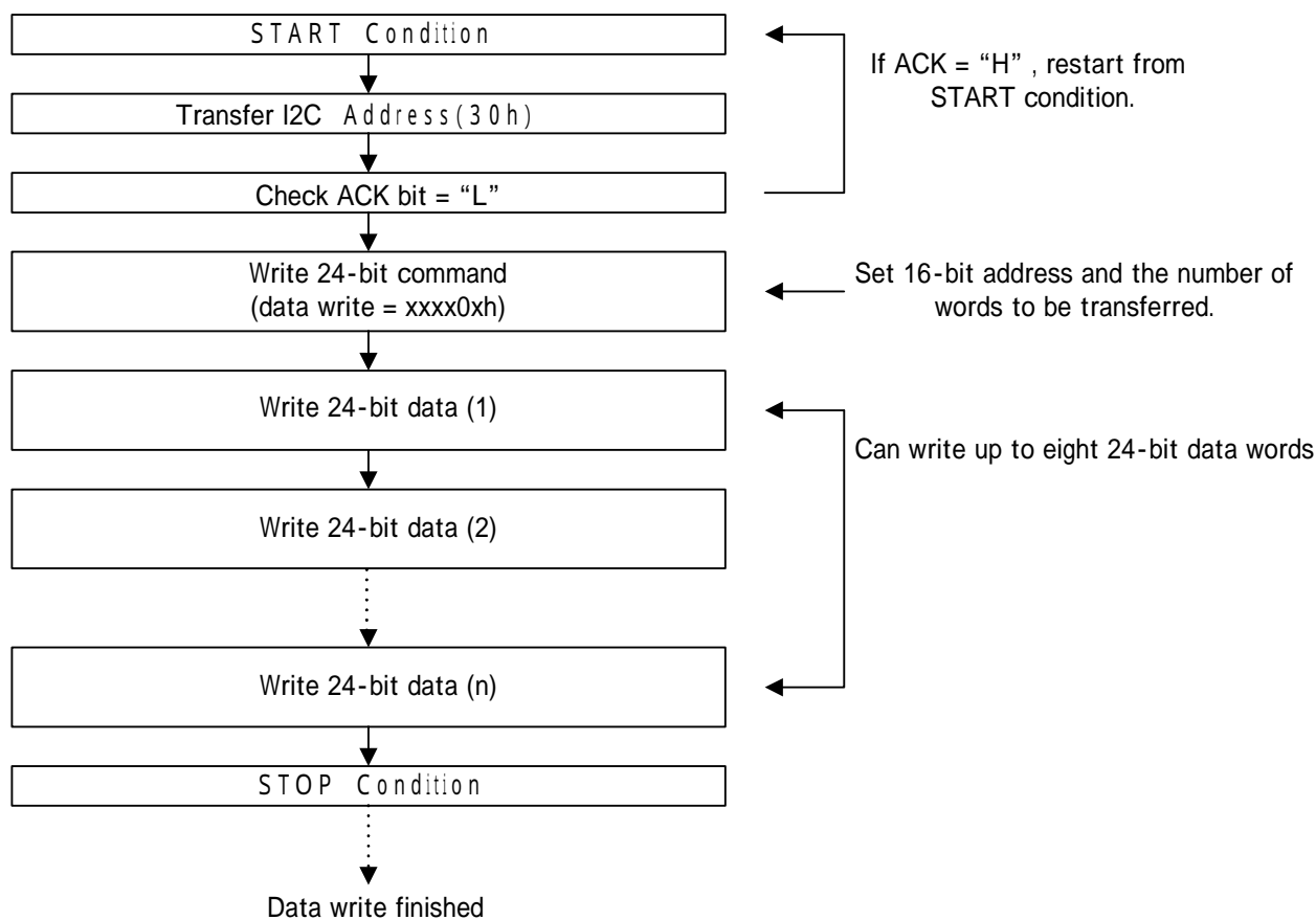
Figure 15 shows the 24-bit Data Write Procedure.
