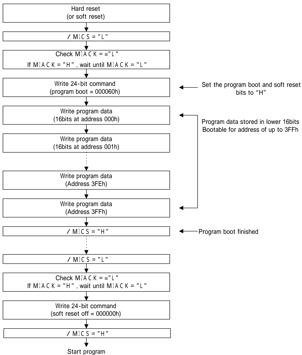
Figure 6 Program Boot and Program Start Procedure
