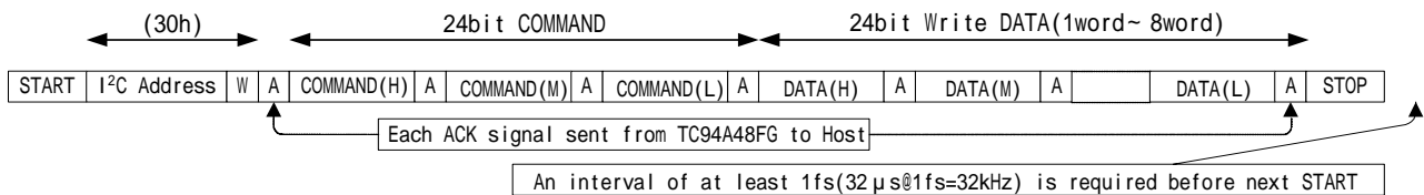
Figure 11 Format for Writing
