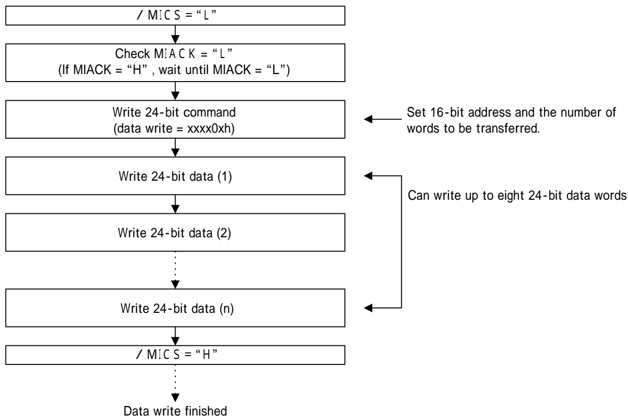
Figure 7 shows the 24-bit data write procedure.
