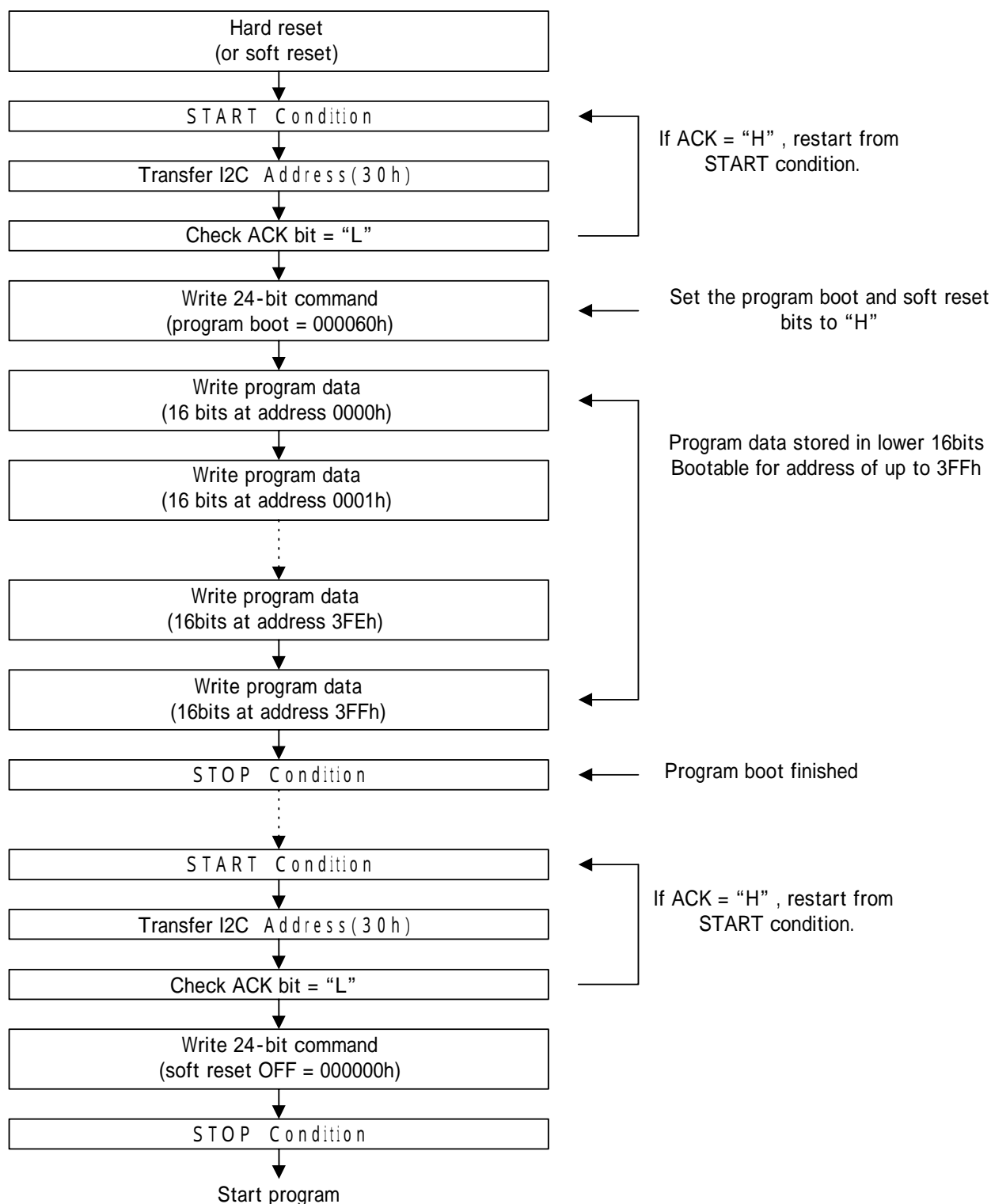
Figure 14 Program Boot and Program Start Procedure
