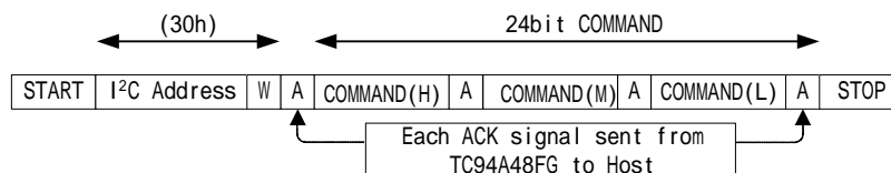
Figure 13 Format for Transferring a Command Only
