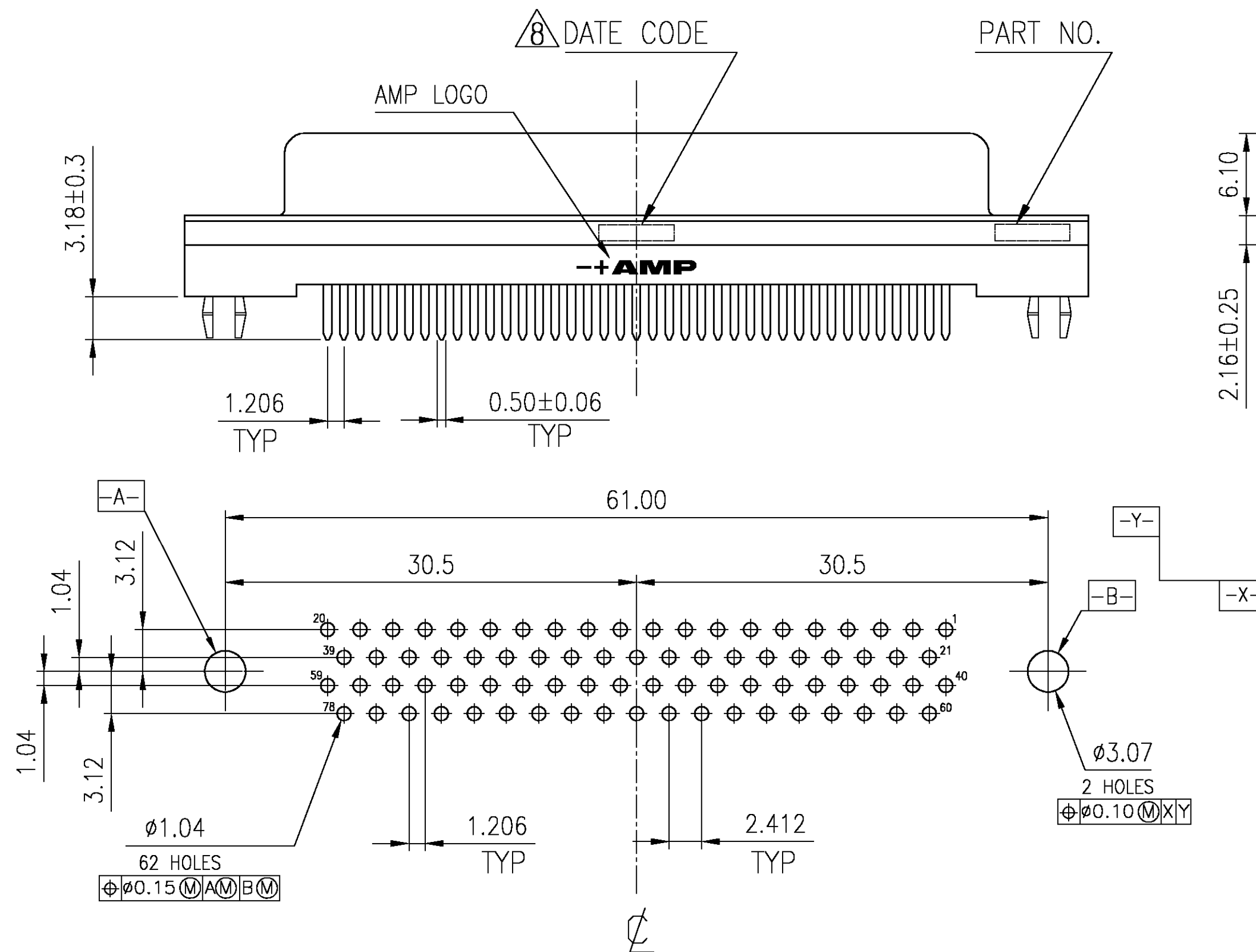
RECOMMENDED PCB LAYOUT
