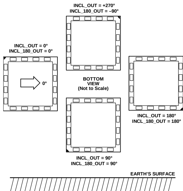
Figure 25. Output Response vs. Orientation
