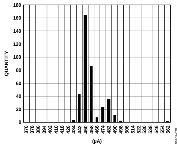
Figure 20. Sleep Mode Power Supply Current Distribution at 25°C/3.3 V
