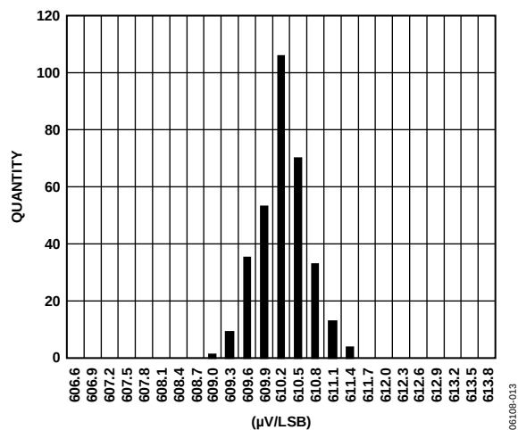
Figure 13. DAC Gain Distribution at 25°C/3.3 V
