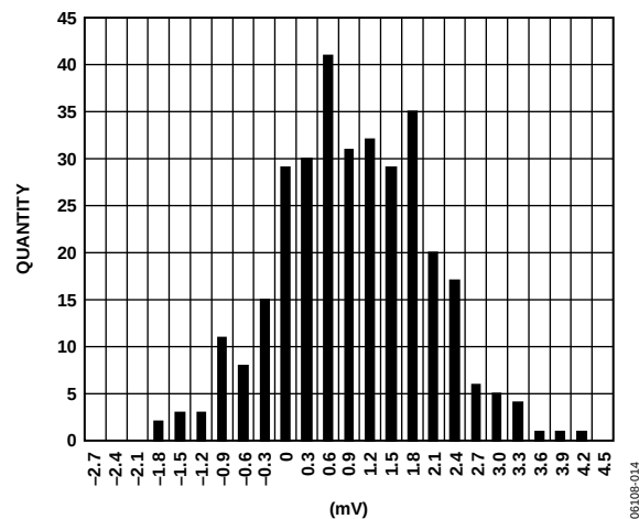
Figure 14. DAC Offset Distribution at 25°C/3.3 V
