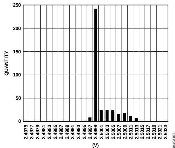
Figure 16. VREF Distribution at 25°C/3.3 V
