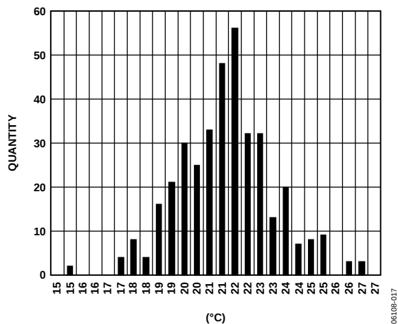
Figure 17. Temperature Distribution at 25°C/3.3 V
