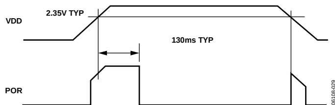
Figure 33. Internal Power-On Reset Operation
