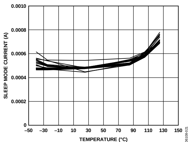
Figure 21. Sleep Mode Current vs. Temperature at 3.3 V
