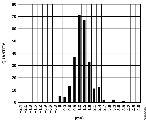
Figure 10. ADC Offset Distribution at 25°C/3.3 V
