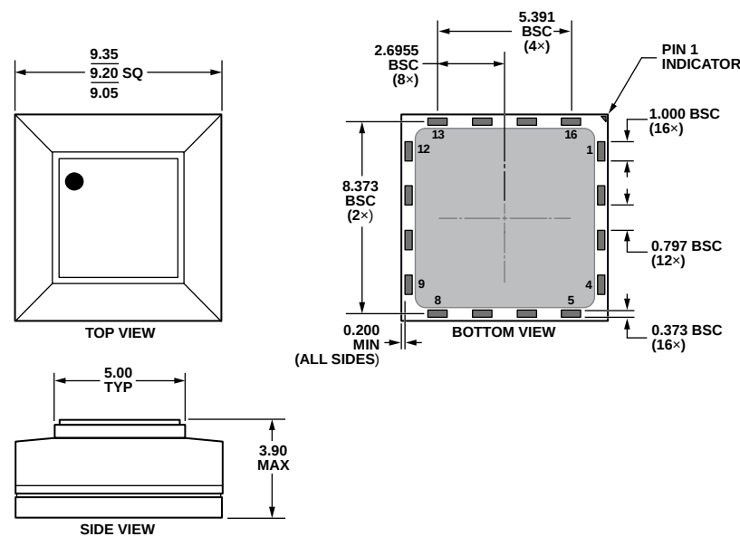
Figure 36. 16-Terminal Land Grid Array [LGA] (CC-16-2) Dimensions shown in millimeters
