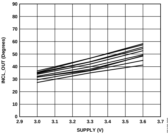
Figure 8. Self-Test Shift vs. Supply at 25°C
