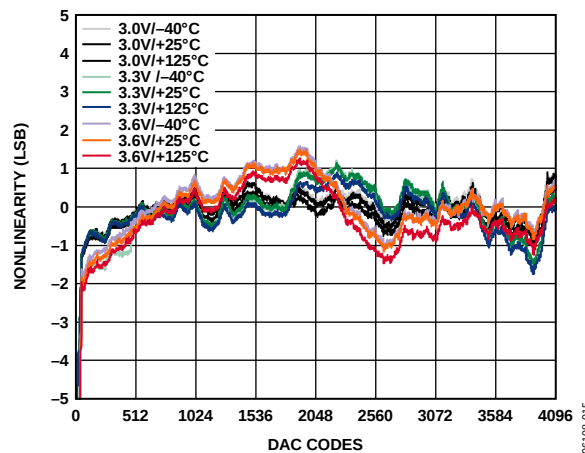
Figure 15. Typical DAC Integral Nonlinearity
