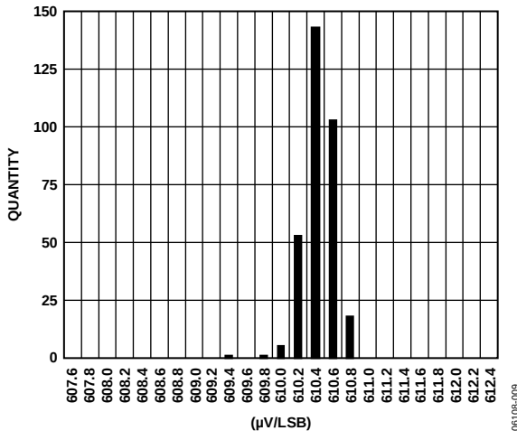
Figure 9. ADC Gain Distribution at 25°C/3.3 V
