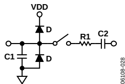
Figure 32. Equivalent Analog Input Circuit Conversion Phase: Switch Open Track Phase: Switch Closed
