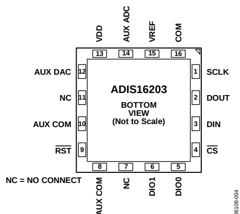
Figure 4. Pin Configuration
