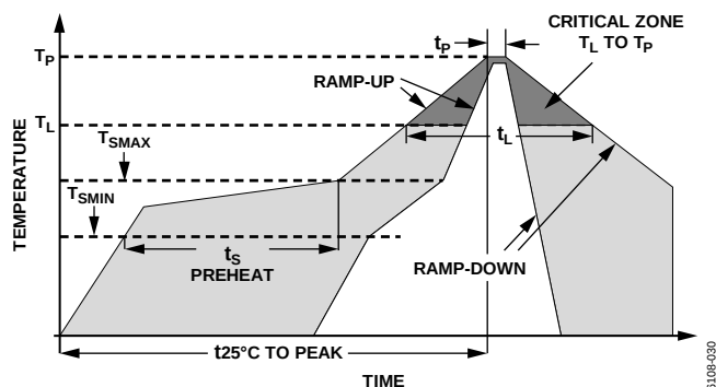
Figure 34. Acceptable Solder Reflow Profiles
