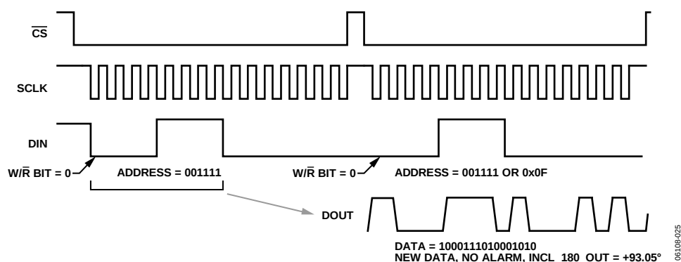
Figure 28. SPI Sequence Reading INCL_OUT When Incline Angle = 93.05^\circ
