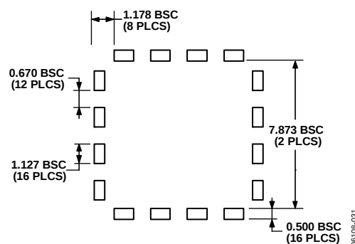
Figure 35. Example Pad Layout
