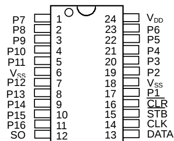
NJU3716L/M
