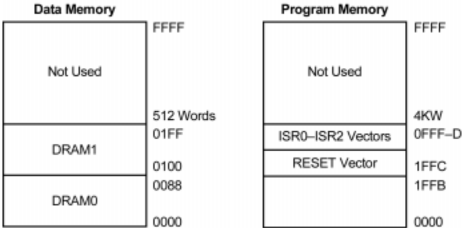
Figure 16. Memory Map
