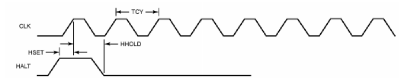
Figure 12. HALT Timing
