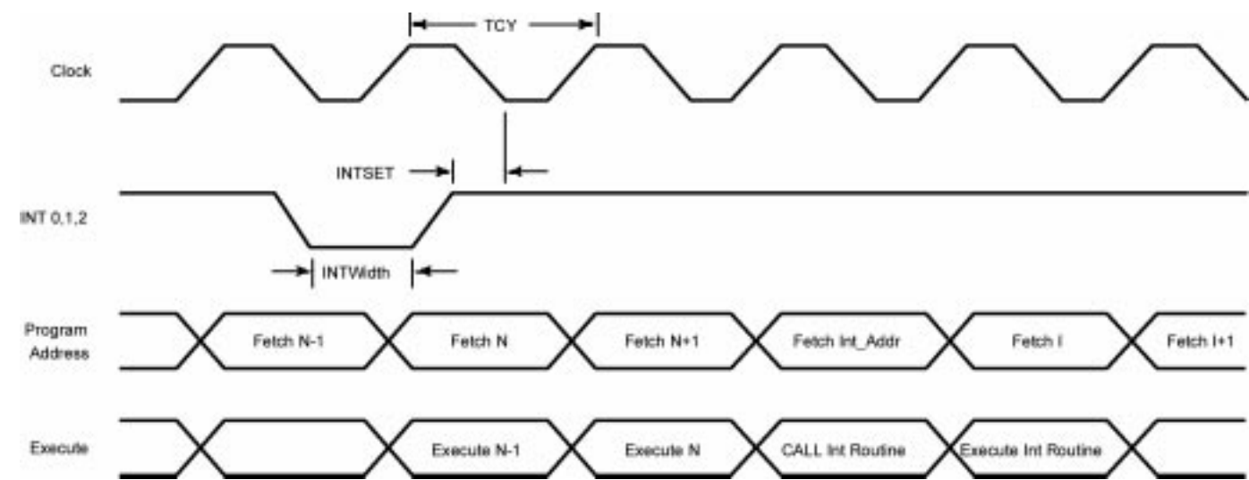
Figure 11. Interrupt Timing
