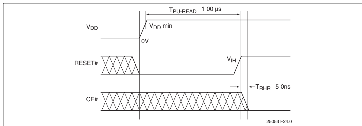
Figure 5: Power-Up Diagram
