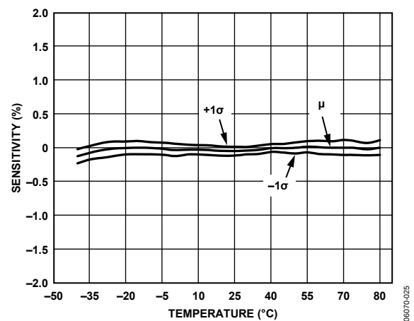
Figure 11. Sensitivity vs. Temperature, ADIS16255
