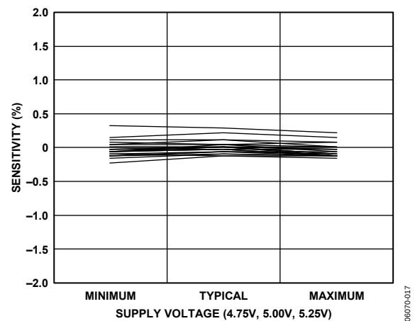
Figure 12. Sensitivity vs. Supply Voltage
