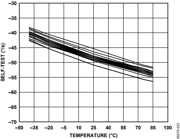
Figure 18. Negative Self-Test vs. Temperature
