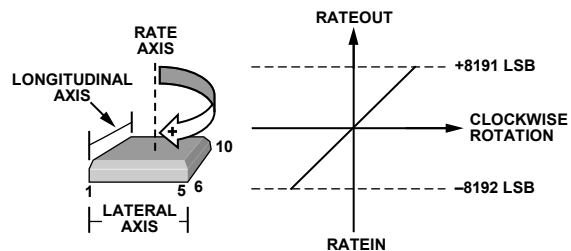
Figure 4. RATEOUT Level Increase with Clockwise Rotation Increase
