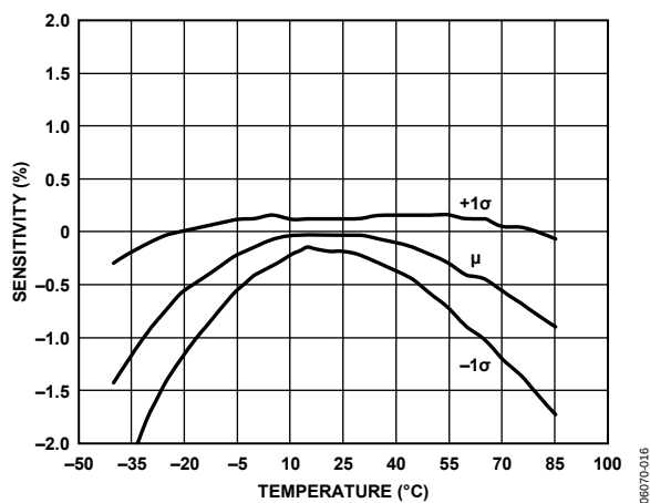
Figure 8. Sensitivity vs. Temperature, ADIS16250
