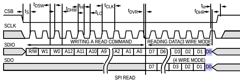
FIGURE 38. READ TIMING
