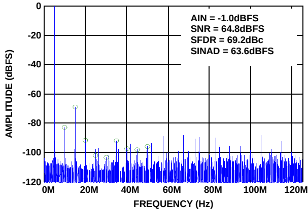
FIGURE 19. SINGLE-TONE SPECTRUM @ 495MHz
