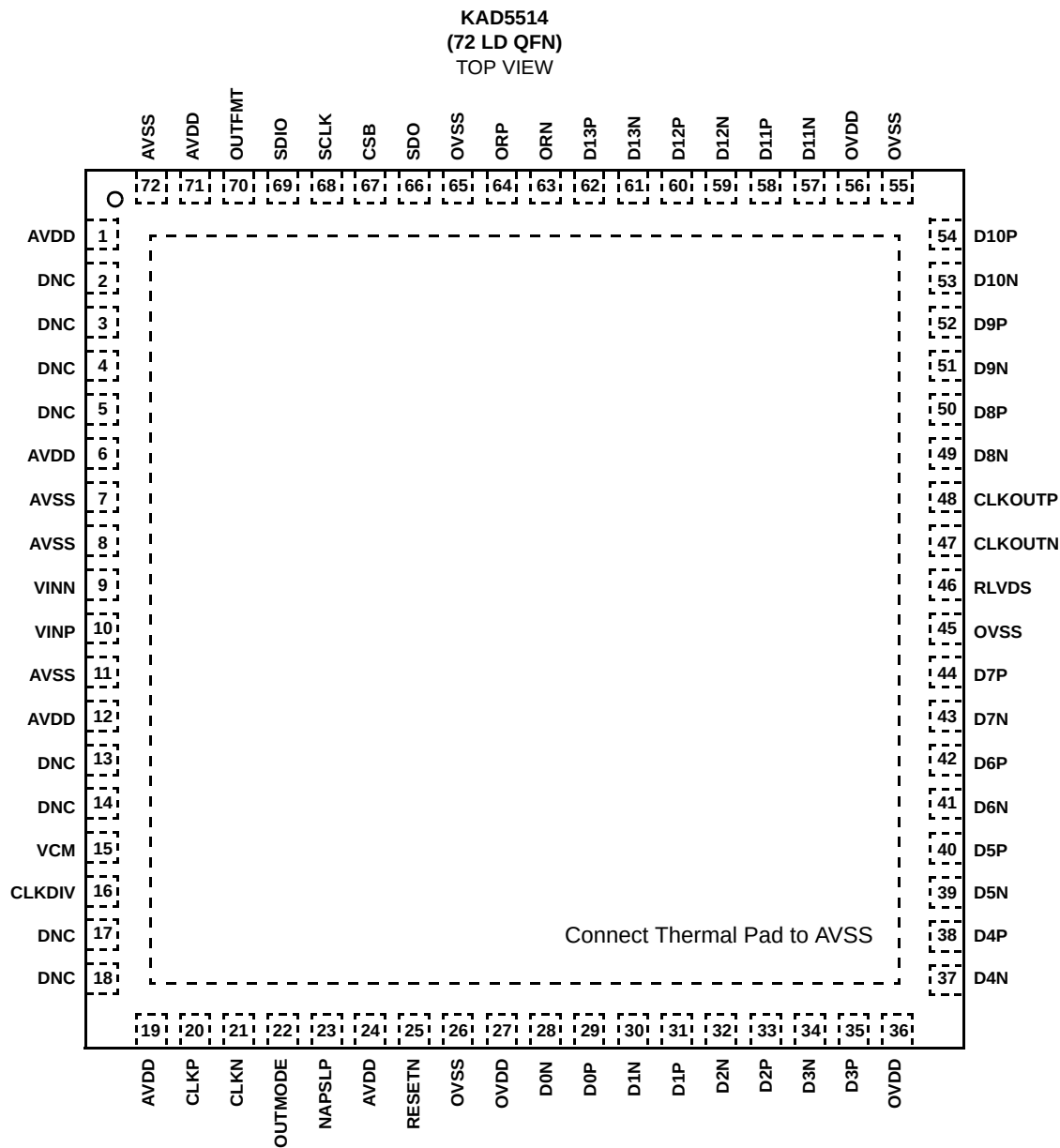
FIGURE 3. PIN CONFIGURATION
