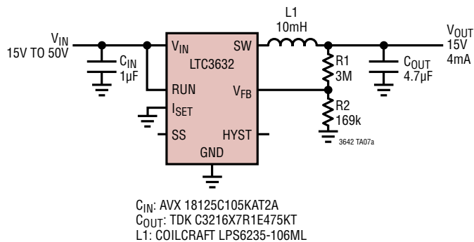
High Efficiency 15V, 4mA Regulator
