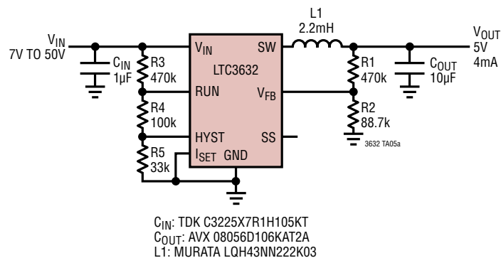
Small Size, Limited Peak Current, 4mA Regulator
