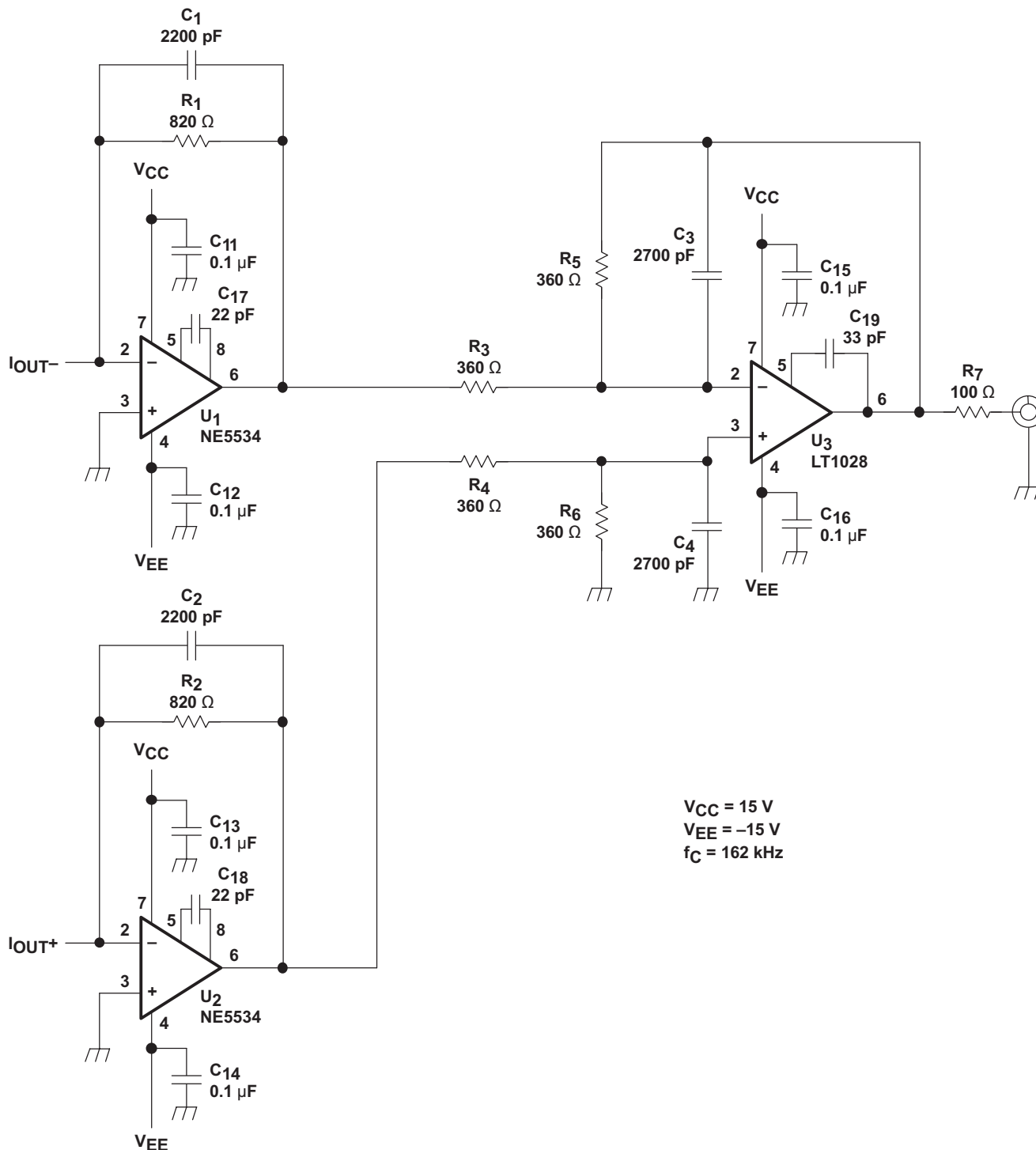
Figure 26. Measurement Circuit, V_{OUT} = 4.5-V_{RMS}
