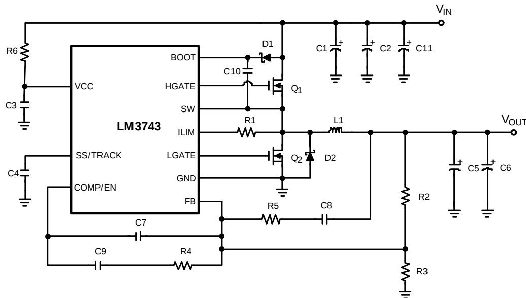
Figure 56. Schematic
