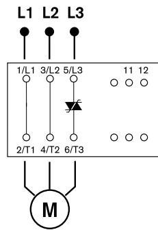
Three phase operation
