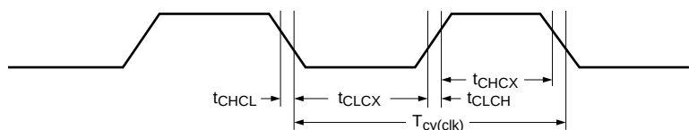
Fig 41. External clock timing (with an amplitude of at least V_{i(RMS)} = 200 \text{ mV} )
