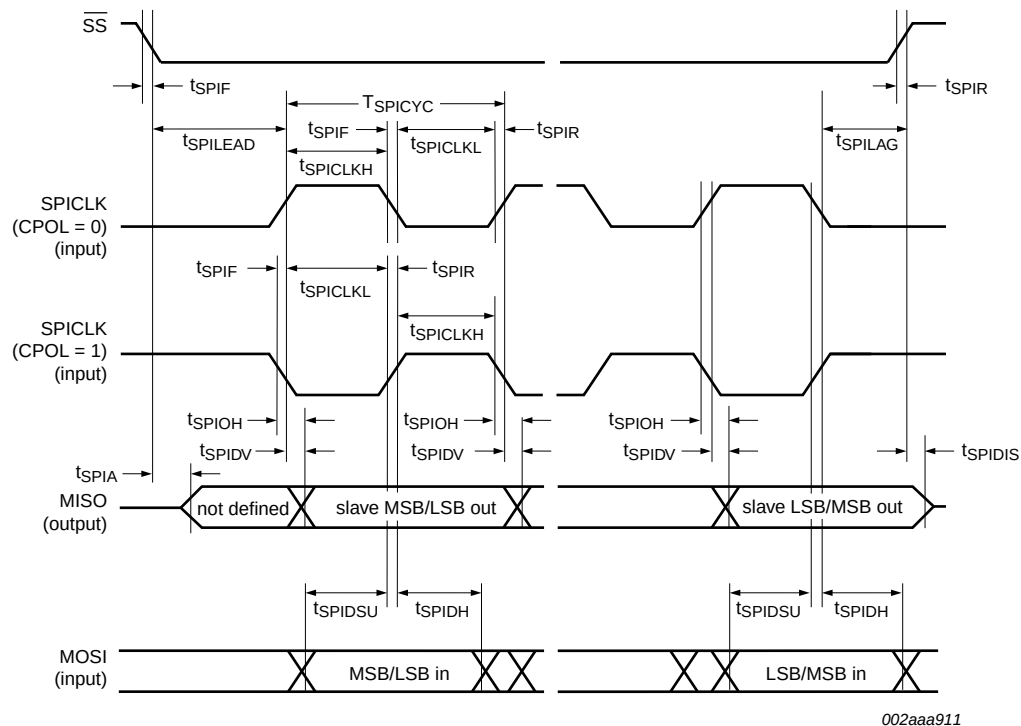
Fig 46. SPI slave timing (CPHA = 1)
