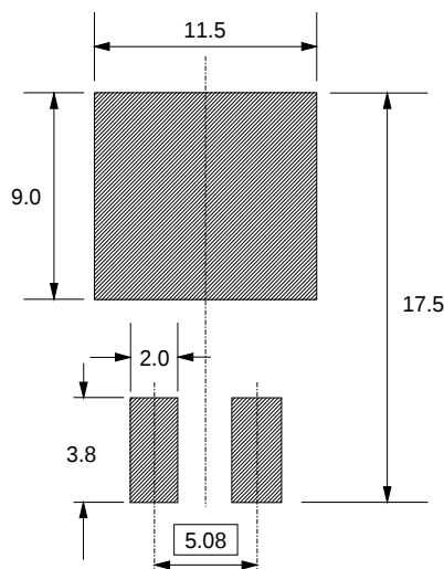
Fig.18. SOT404 : soldering pattern for surface mounting.
