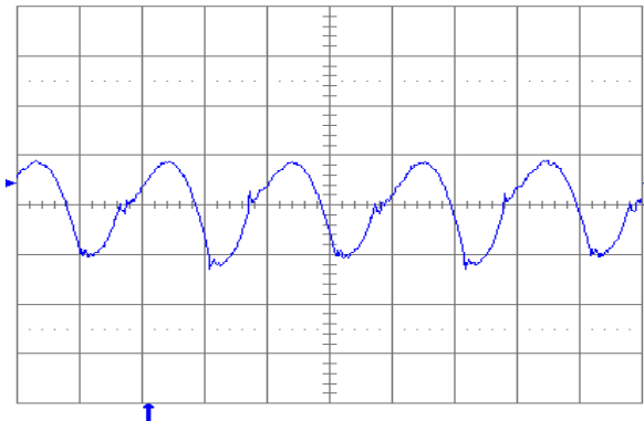
Figure 1.5V.19. Output voltage ripple (20 mV/div.) at full rated load current into a resistive load with C_o = 10 \mu\text{F} tantalum + 1 \mu\text{F} ceramic and V_{in} = 48 \text{ V} . Time scale: 1 \mu\text{s}/\text{div} .
