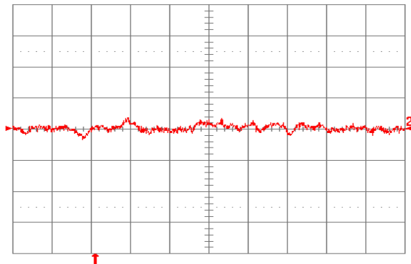
Figure 1.0V.22. Input reflected ripple current, i_s (10 mA/div.), measured through 10\ \mu\text{H} at the source at full rated load current and V_{in} = 48\ \text{V} . Refer to Fig. 1.0V.20 for test setup. Time scale: 1\ \mu\text{s}/\text{div} .
