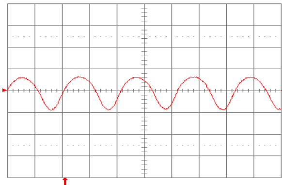
Figure 1.5V.21. Input reflected ripple current, i_c (100 mA/div.), measured at input terminals at full rated load current and V_{in} = 48 \text{ V} . Refer to Fig. 1.5V.20 for test setup. Time scale: 1 \mu\text{s}/\text{div} .
