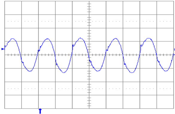
Figure 2.5V.19. Output voltage ripple (20 mV/div.) at full rated load current into a resistive load with C_o = 10\ \mu\text{F} tantalum + 1\ \mu\text{F} ceramic and V_{in} = 48\ \text{V} . Time scale: 1\ \mu\text{s}/\text{div} .
