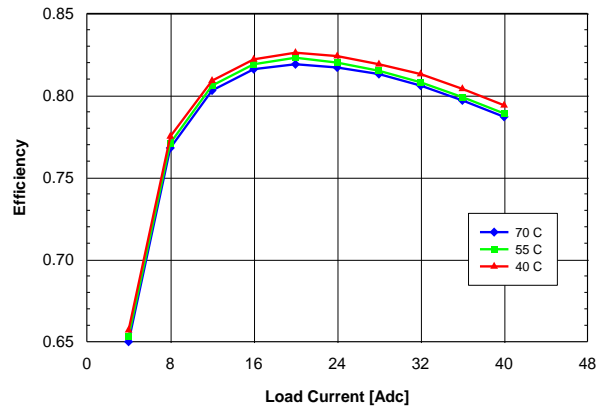
Figure 1.0V.12. Efficiency vs. load current and ambient temperature for QME48T40010 converter mounted horizontally with V_{in} = 48 V and air flowing from pin 1 to pin 3 at a rate of 200 LFM (1.0 m/s).
