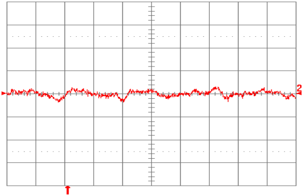
Figure 1.8V.22. Input reflected ripple current, i_s (10 mA/div.), measured through 10\ \mu\text{H} at the source at full rated load current and V_{in} = 48\ \text{V} . Refer to Fig. 1.8V.20 for test setup. Time scale: 1\ \mu\text{s}/\text{div} .
