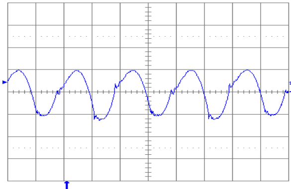
Figure 1.8V.19. Output voltage ripple (20mV/div.) at full rated load current into a resistive load with C_o = 10\ \mu\text{F} tantalum + 1\ \mu\text{F} ceramic and V_{in} = 48\ \text{V} . Time scale: 1\ \mu\text{s}/\text{div} .
