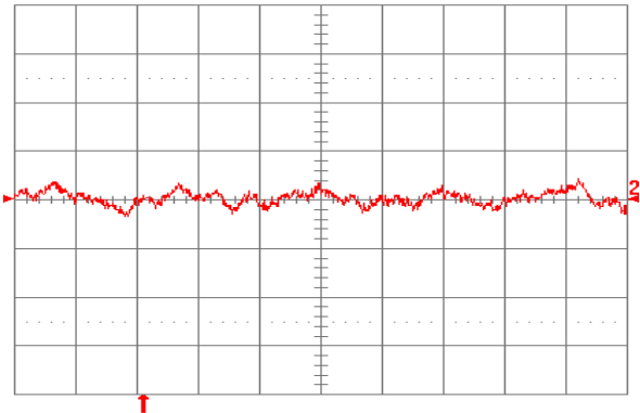
Figure 2.5V.22. Input reflected ripple current, i_s (10 mA/div.), measured through 10\ \mu\text{H} at the source at full rated load current and V_{in} = 48\ \text{V} . Refer to Fig. 2.5V.20 for test setup. Time scale: 1\ \mu\text{s}/\text{div} .
