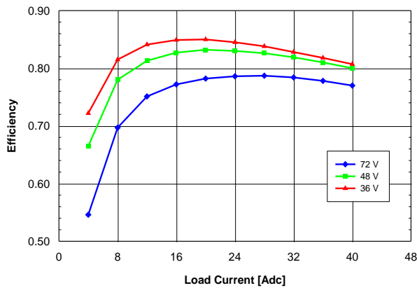
Figure 1.0V.11. Efficiency vs. load current and input voltage for QME48T40010 converter mounted horizontally with air flowing from pin 1 to pin 3 at a rate of 300 LFM (1.5 m/s) and T_a = 25 °C.
