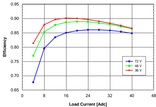
Figure 1.8V.11. Efficiency vs. load current and input voltage for QME48T40018 converter mounted horizontally with air flowing from pin 1 to pin 3 at a rate of 300 LFM (1.5 m/s) and T_a = 25^{\circ}\text{C} .
