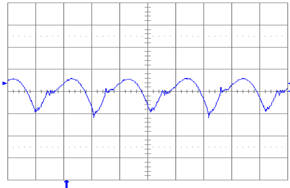
Figure 1.0V.19. Output voltage ripple (20 mV/div.) at full rated load current into a resistive load with C_o = 10\ \mu\text{F} tantalum + 1\ \mu\text{F} ceramic and V_{in} = 48\ \text{V} . Time scale: 1\ \mu\text{s}/\text{div} .
