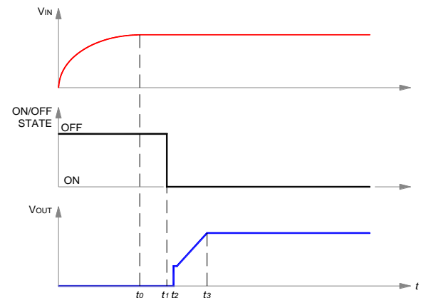
Figure 6. Startup scenario #2.
