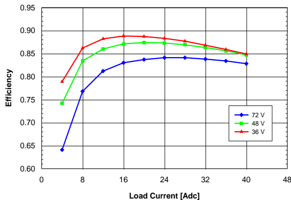
Figure 1.5V.11. Efficiency vs. load current and input voltage for QME48T40015 converter mounted horizontally with air flowing from pin 1 to pin 3 at a rate of 300 LFM (1.5 m/s) and T_a = 25^\circ\text{C} .
