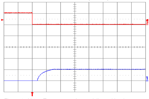
Figure 1.0V.16. Turn-on transient at full rated load current (resistive) plus 10,000 \mu\text{F} at V_{in} = 48\text{ V} , triggered via ON/OFF pin. Top trace: ON/OFF signal (5 V/div.). Bottom trace: output voltage (1 V/div.). Time scale: 2 ms/div.
