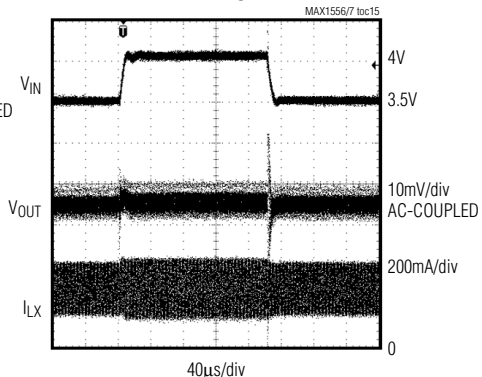
LINE TRANSIENT
