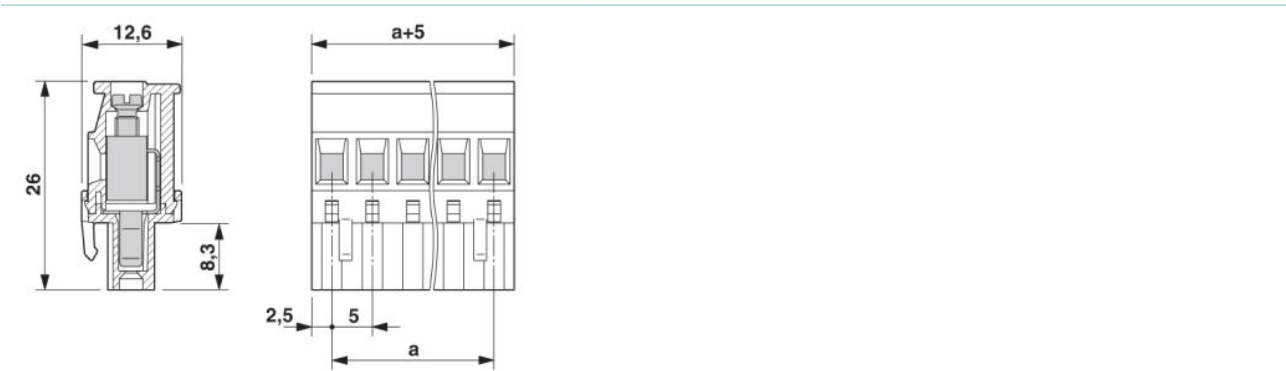
Dimensioned drawing
