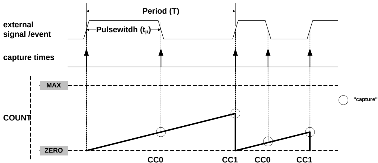
Figure 32-18. PWP Capture
