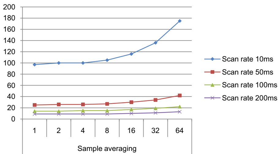
Figure 37-9. Power Consumption [ \mu A] 1 sensor, noise countermeasures Enabled, f=48MHz, Vcc=3.3V
