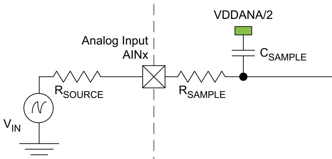
Figure 37-6. ADC Input
