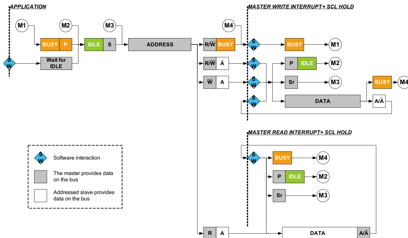
Figure 30-7. I 2 C Master Behavioral Diagram (SCLSM=1)
