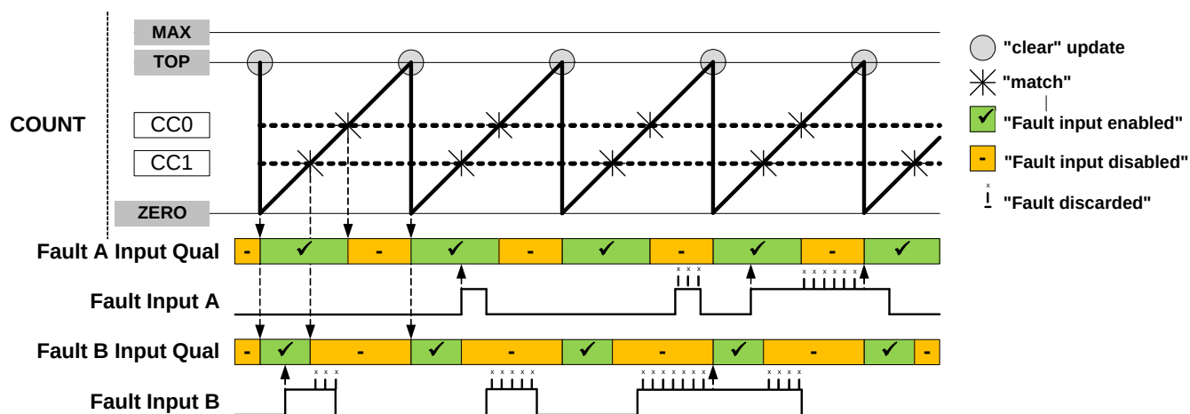
Figure 32-23. Fault Qualification in RAMP1 Operation
