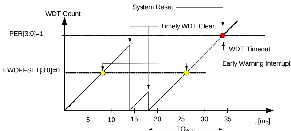
Figure 20-2. Normal-Mode Operation
