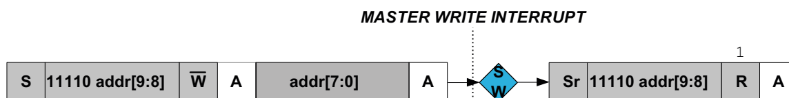
Figure 30-9. 10-Bit Address Transmission for a Read Transaction
