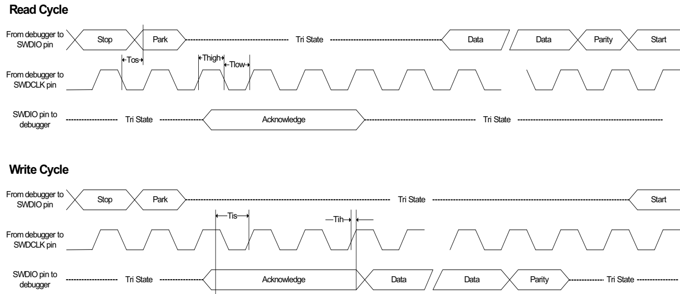
Figure 37-18.SWD Interface Signals
