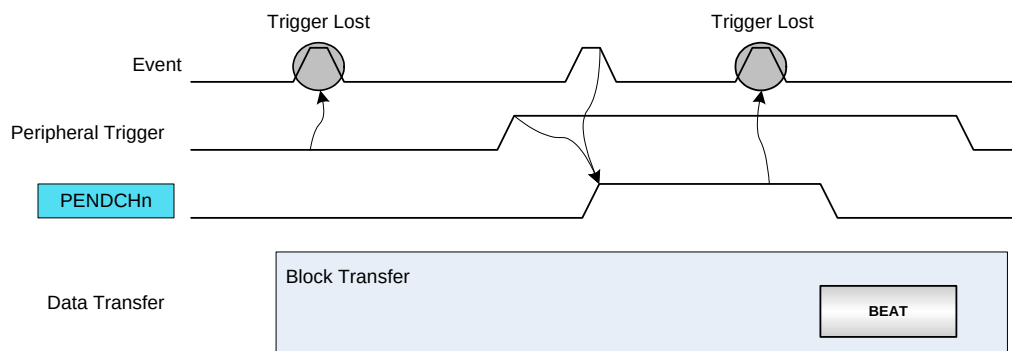
Figure 22-12. Periodic Event with Beat Peripheral Triggers
