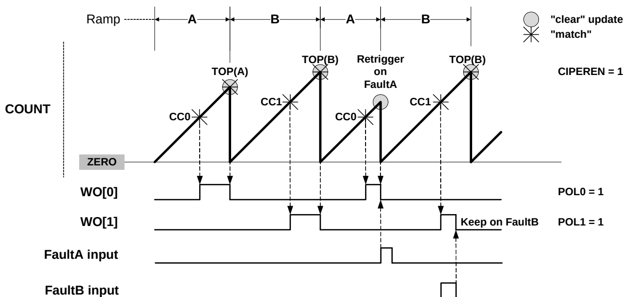
Figure 32-20. RAMP2 Standard Operation
