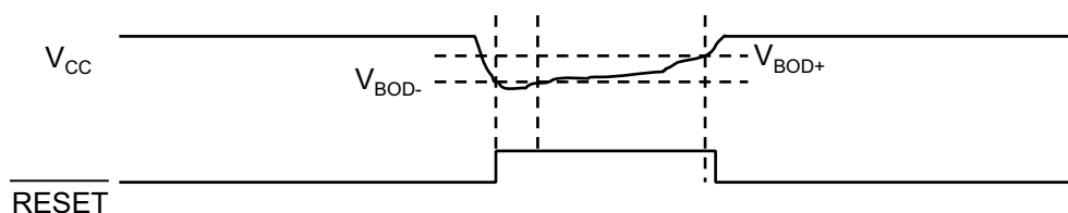
Figure 37-5. BOD33 Hysteresis ON
