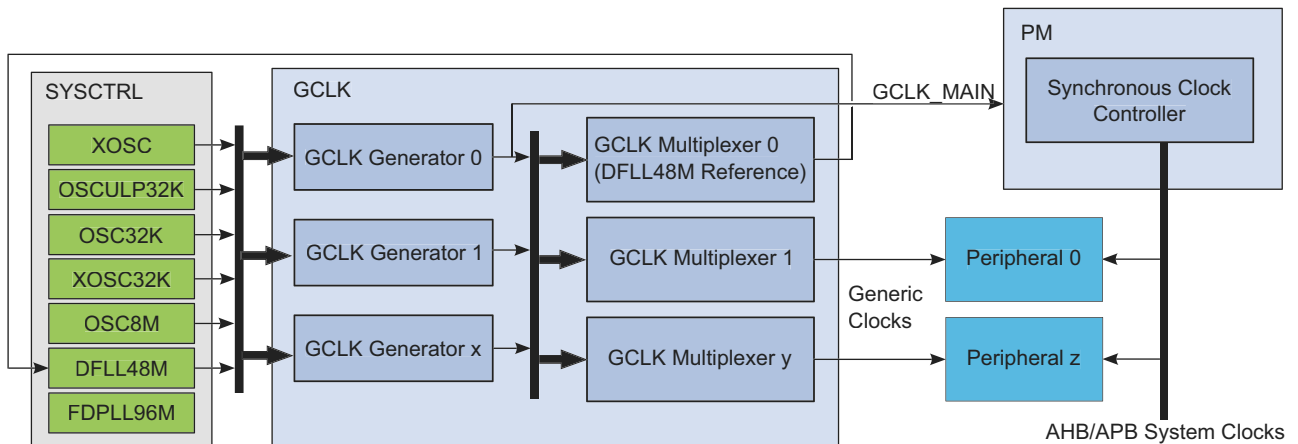
Figure 16-1. Clock distribution
