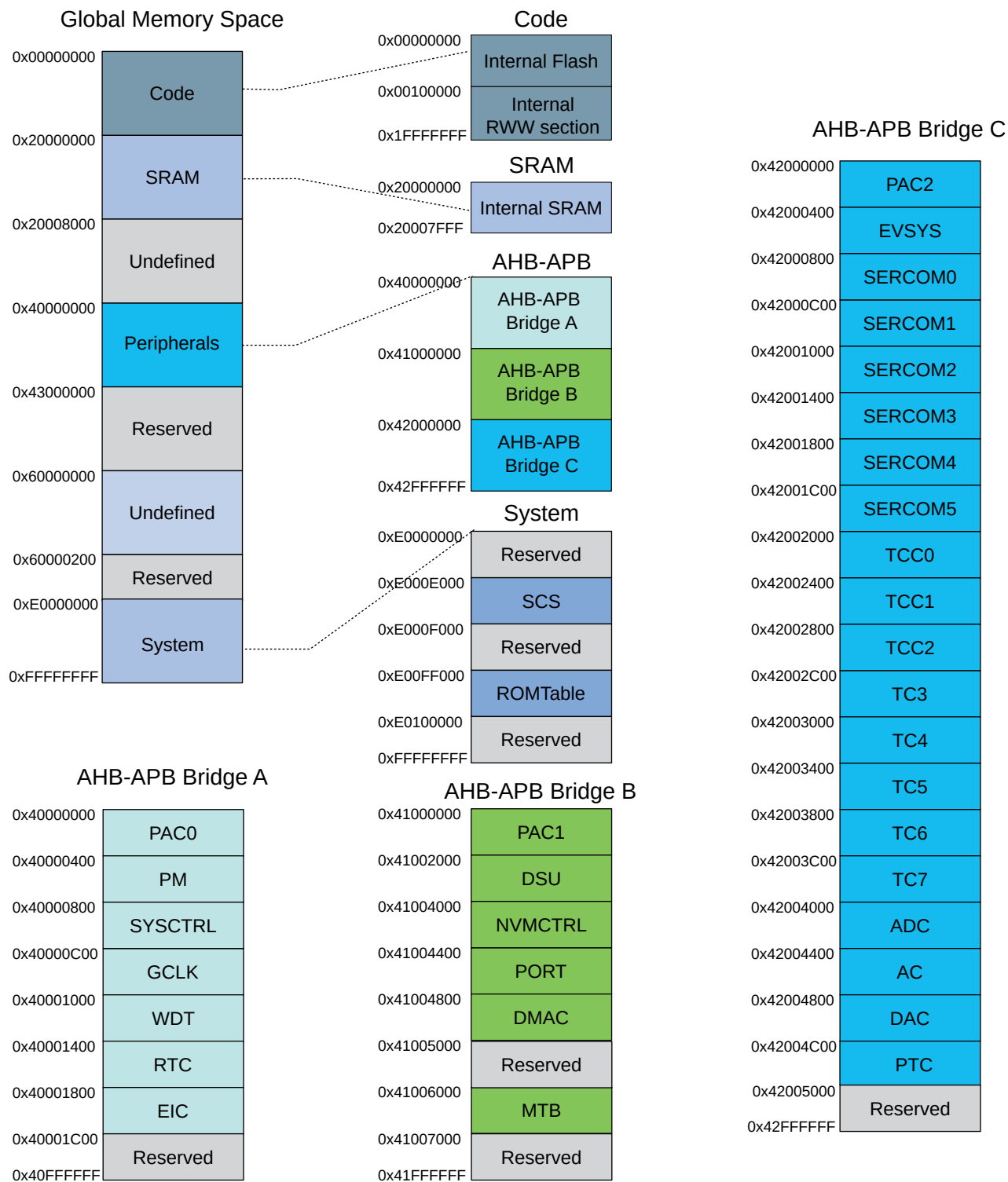
Figure 9-1. Atmel | SMART SAM HA1 A Product Mapping
