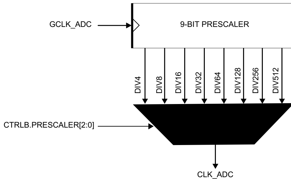
Figure 33-2. ADC Prescaler
