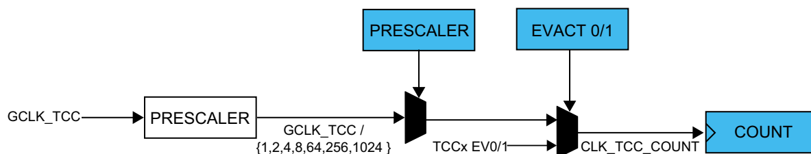
Figure 32-4. Prescaler
