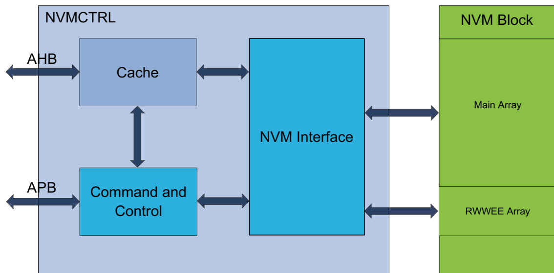
Figure 24-1. Block Diagram
