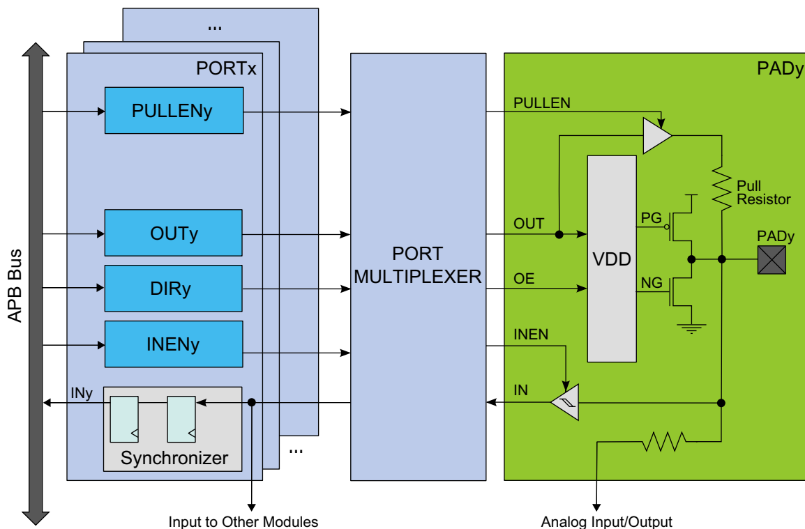
Figure 25-2. Overview of the PORT
