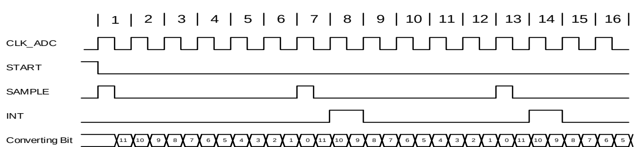
Figure 33-5. ADC Timing for Free Running in Differential Mode without Gain
