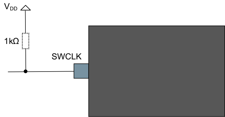
Figure 38-10.SWCLK Circuit Connections
