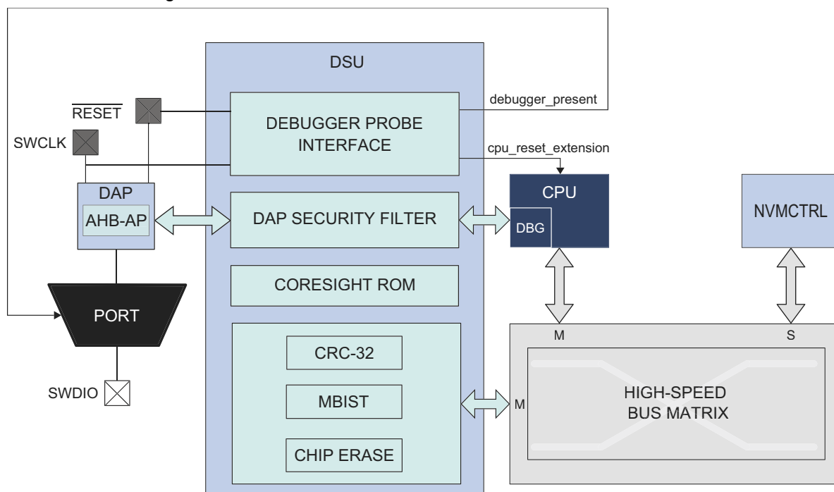
Figure 15-1. DSU Block Diagram
