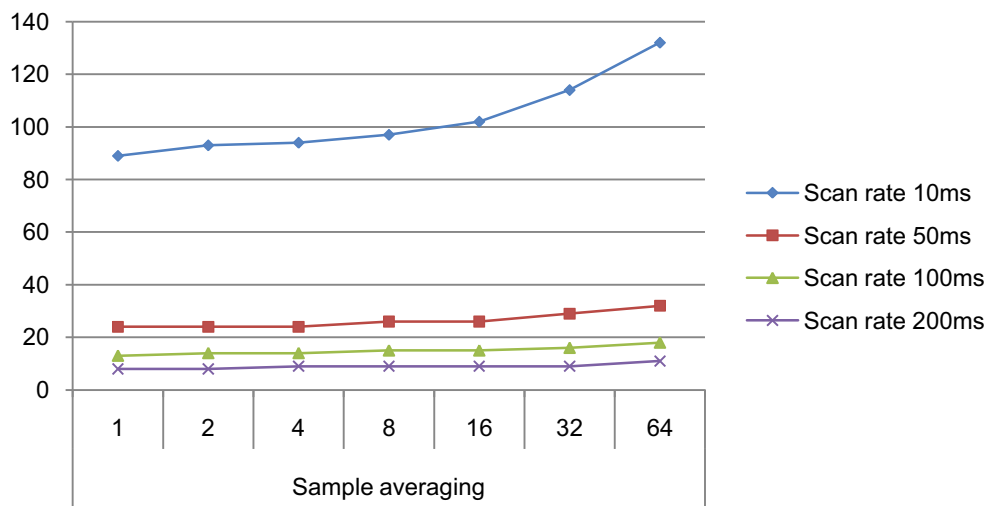
Figure 37-8. Power Consumption [ \mu A] 1 sensor, noise countermeasures disabled, f=48MHz, Vcc=3.3V
