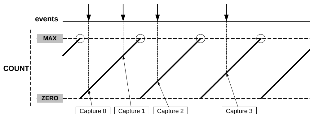
Figure 32-16.Input Capture Timing
