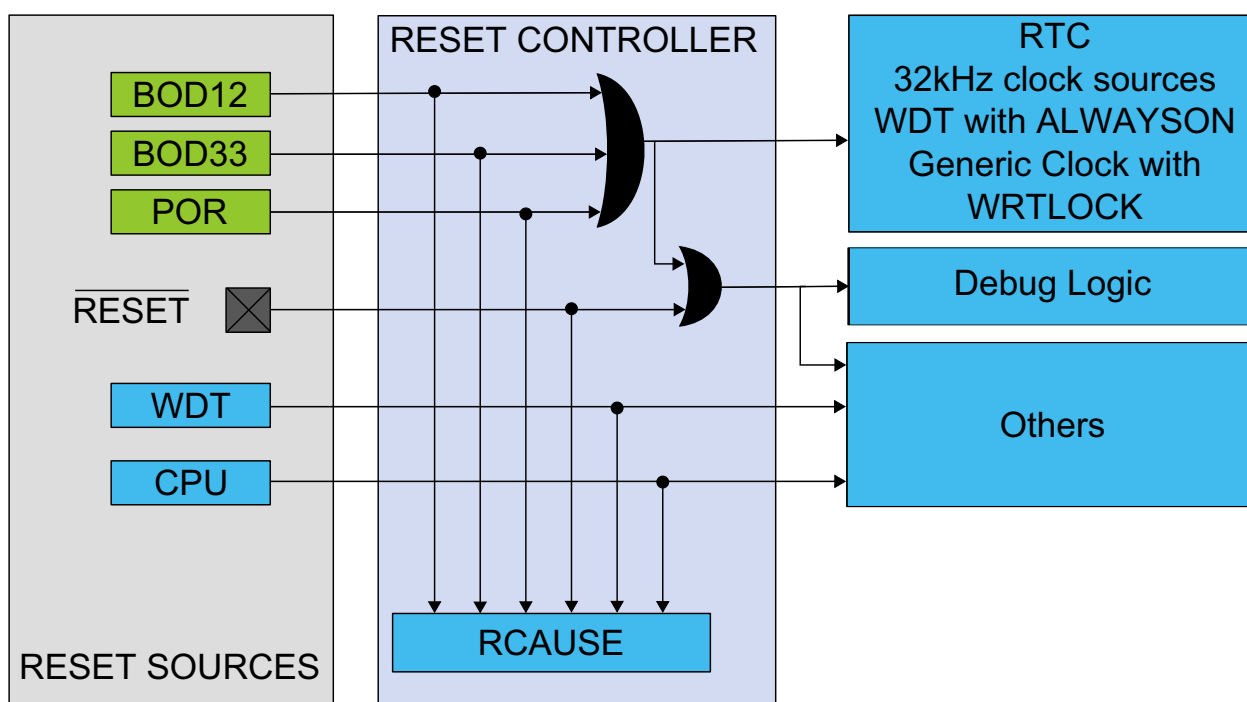
Figure 18-3. Reset Controller
