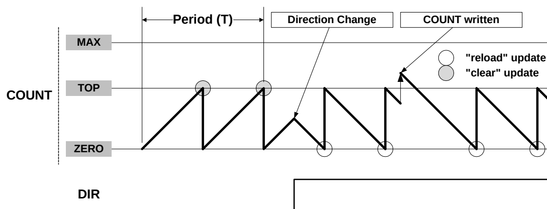
Figure 32-5. Counter Operation
