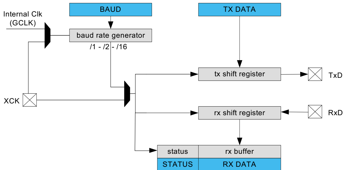
Figure 28-1. USART Block Diagram
