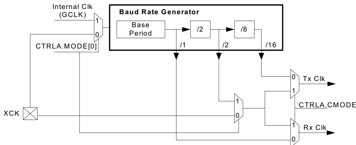
Figure 28-3. Clock Generation
