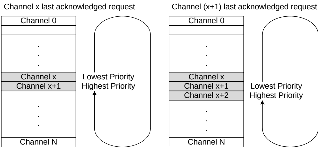
Figure 22-6. Round-Robin Scheduling
