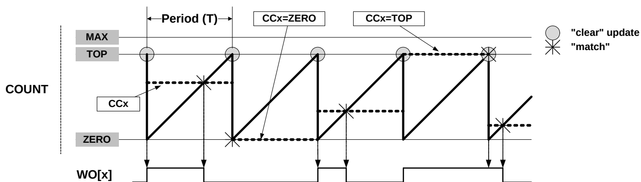
Figure 32-8. Single-Slope PWM Operation
