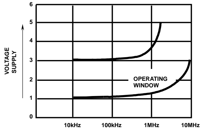
FIGURE 8. WINDOW OF CORRECT OPERATION
