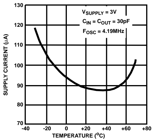
FIGURE 3. SUPPLY CURRENT AS A FUNCTION OF TEMPERATURE
