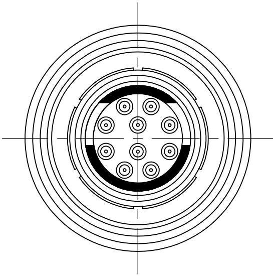
DOUBLE POLARIZATION
