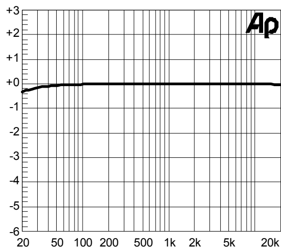
Figure 23 Frequency Response BTL mode, 3V, 80hm
