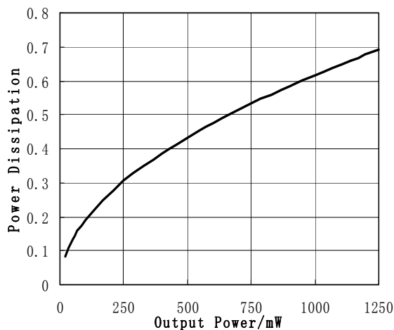
Figure 30 Power Dissipation vs. Output Power BTL mode, 5V, f=1 kHz, RL=80hm, THD+N<=1%
