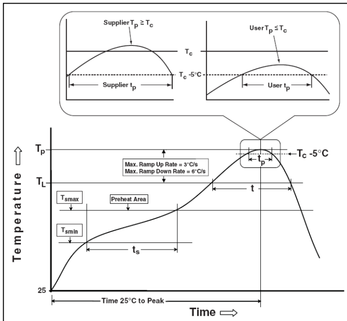
Figure 34 Classification Profile
