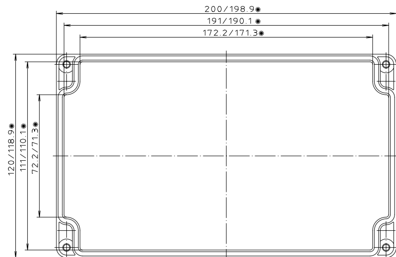
Deckel
