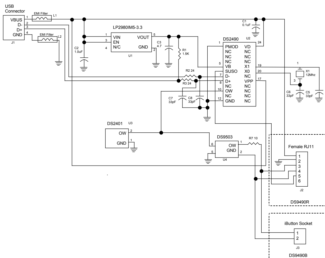
Figure 8. FUNCTIONAL DIAGRAM
