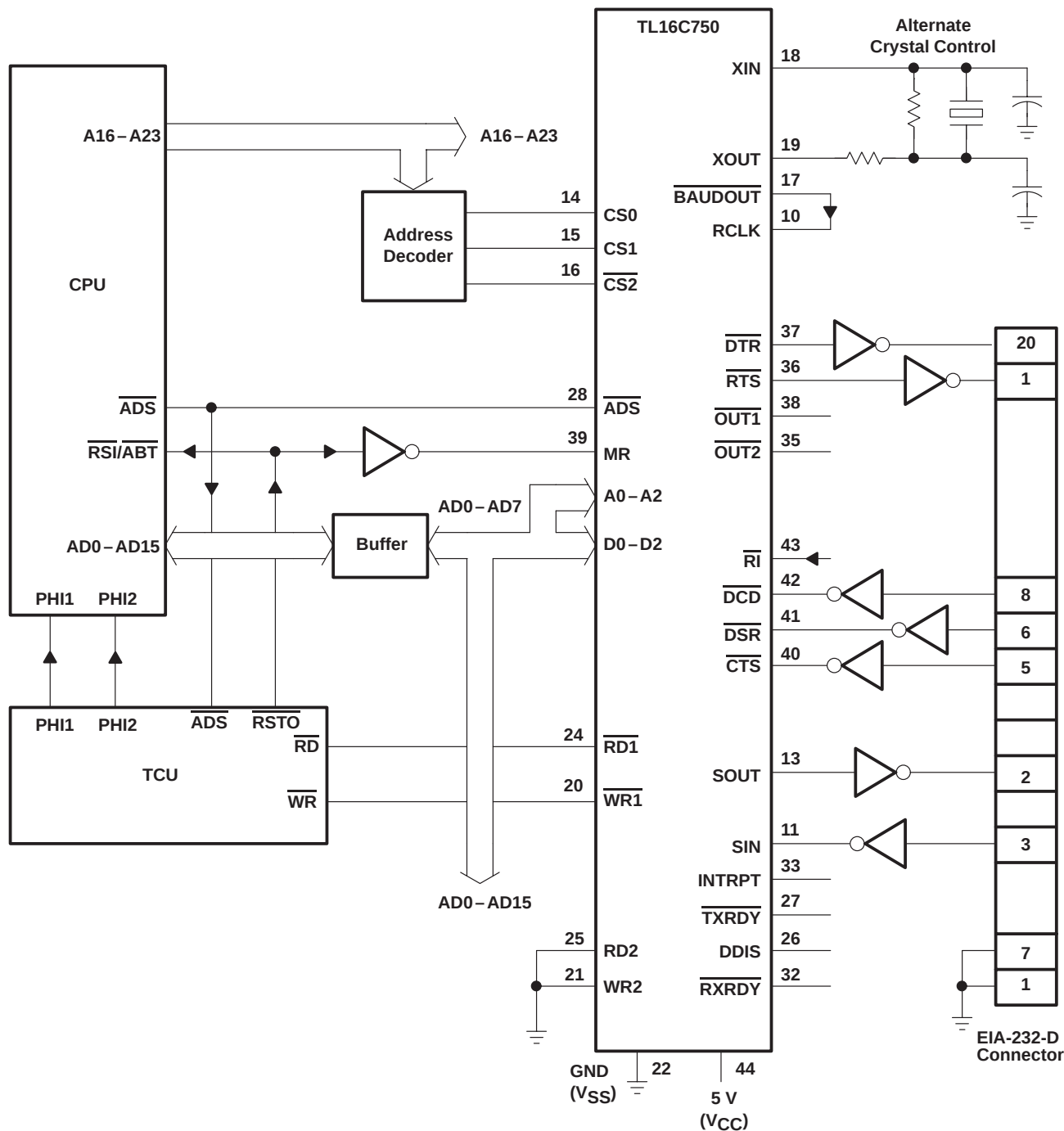
Figure 20. Typical TL16C750 Connection to a CPU
