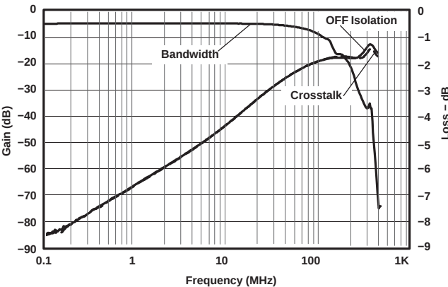
Figure 8. Frequency Response
