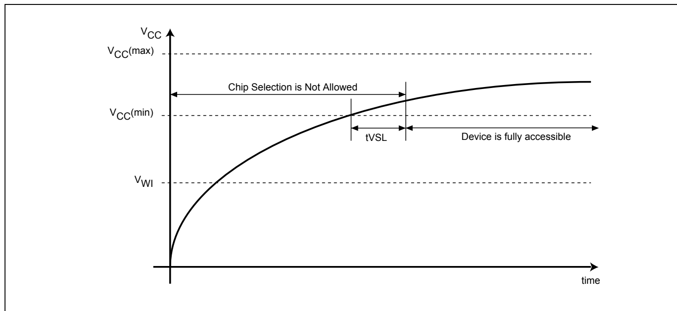
Figure 47. Power-up Timing
