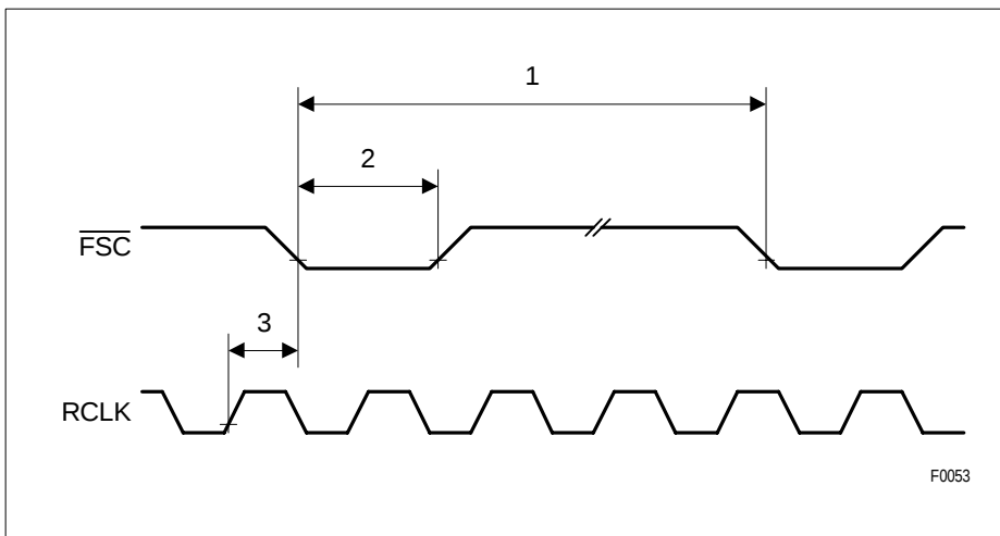
Figure 32 FSC Timing
