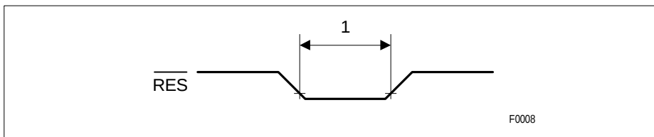
Figure 22 Reset Timing
