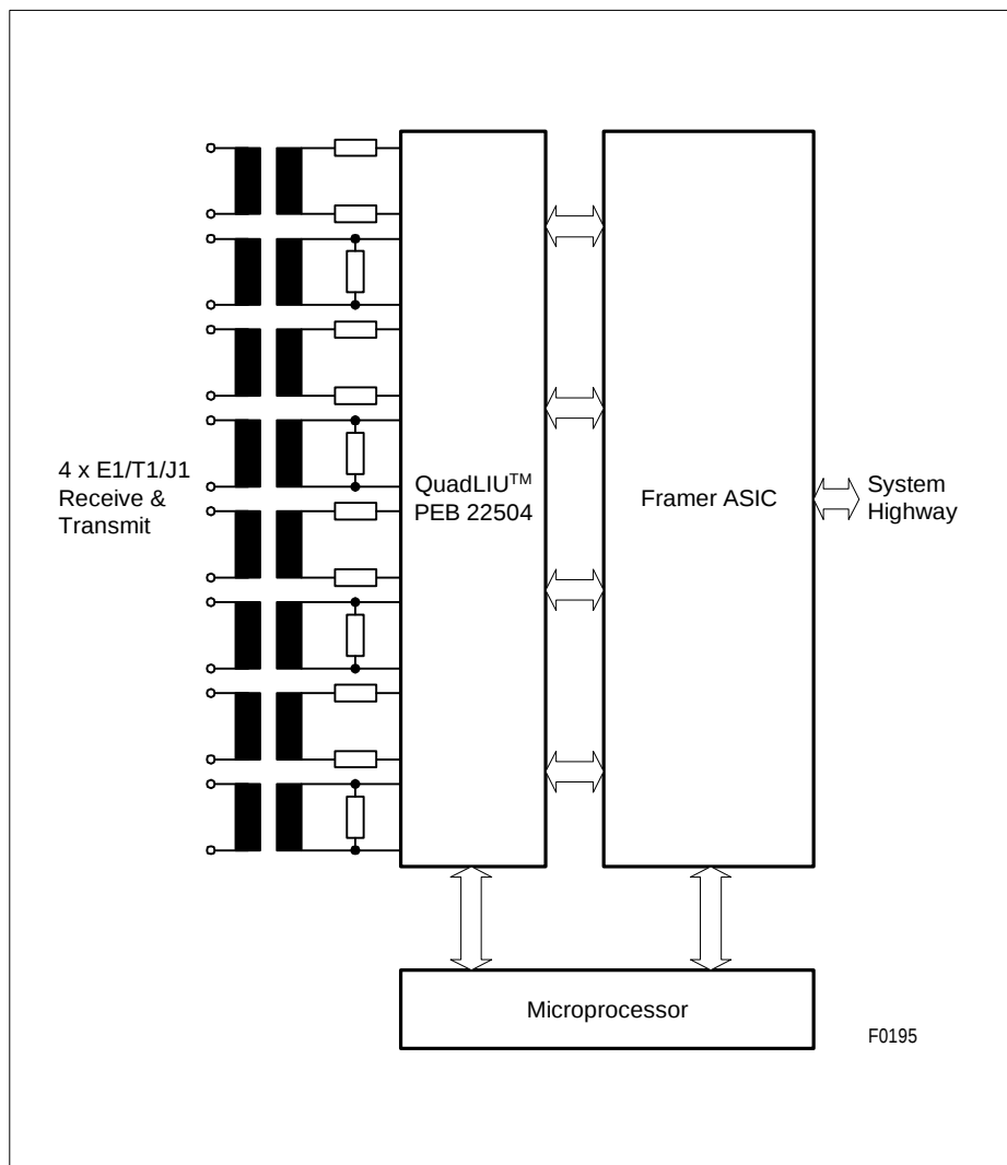
Figure 2 QuadLIU Application
