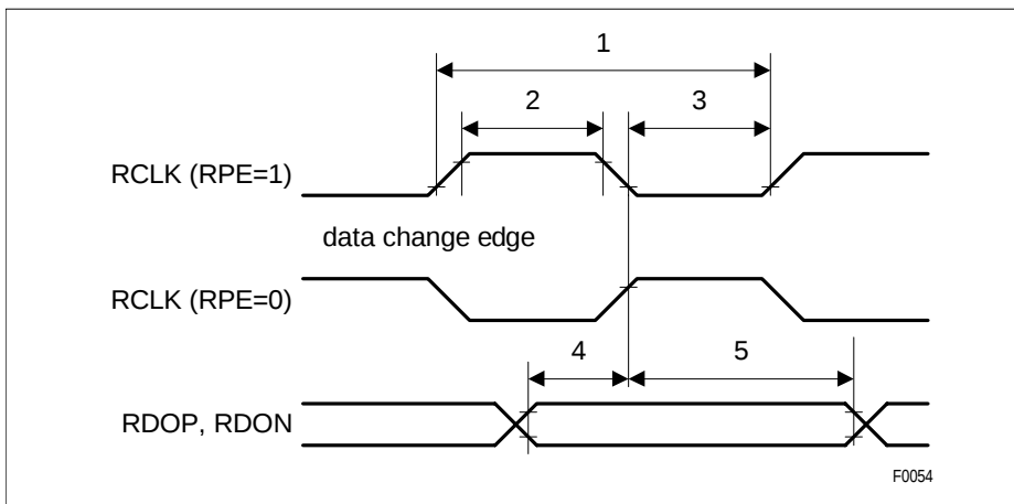
Figure 30 RCLK Output Timing
