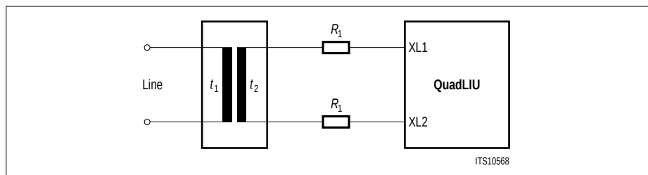
Figure 13 Transmitter Configuration
