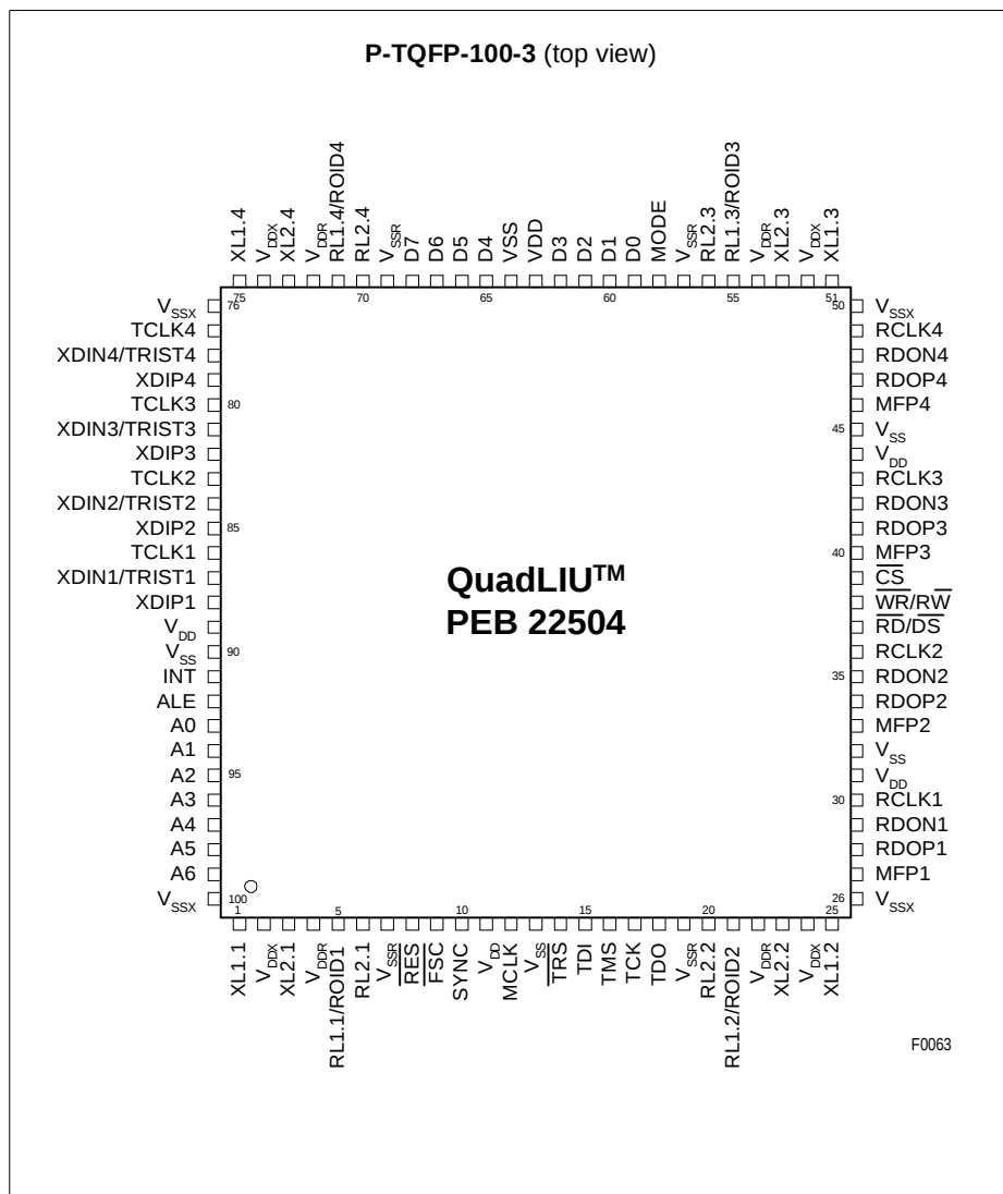
Figure 4 Pin Configuration
