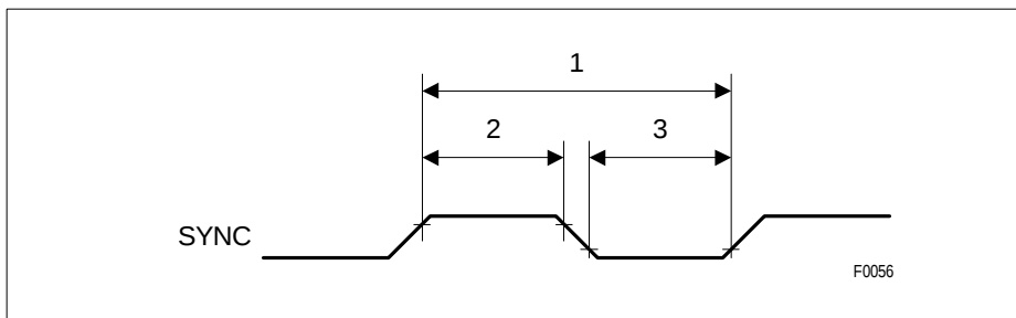
Figure 31 SYNC Timing
