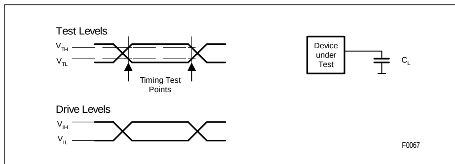
Figure 36 Input/Output Waveforms for AC Testing
