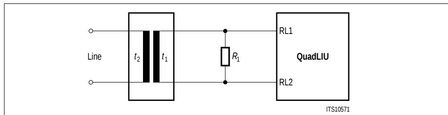
Figure 9 Receiver Configuration
