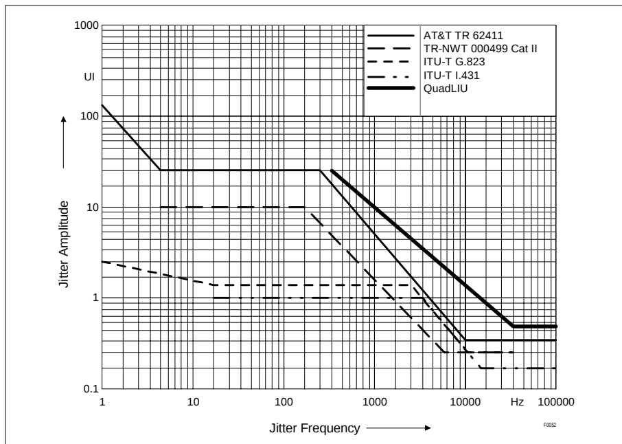
Figure 12 Jitter Tolerance
