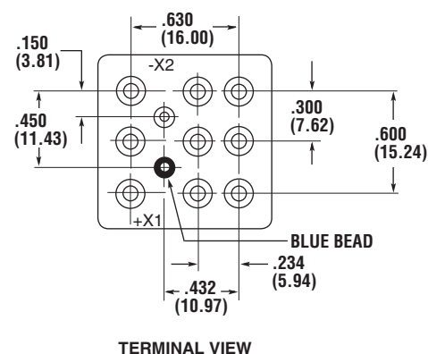
TERMINAL VIEW
