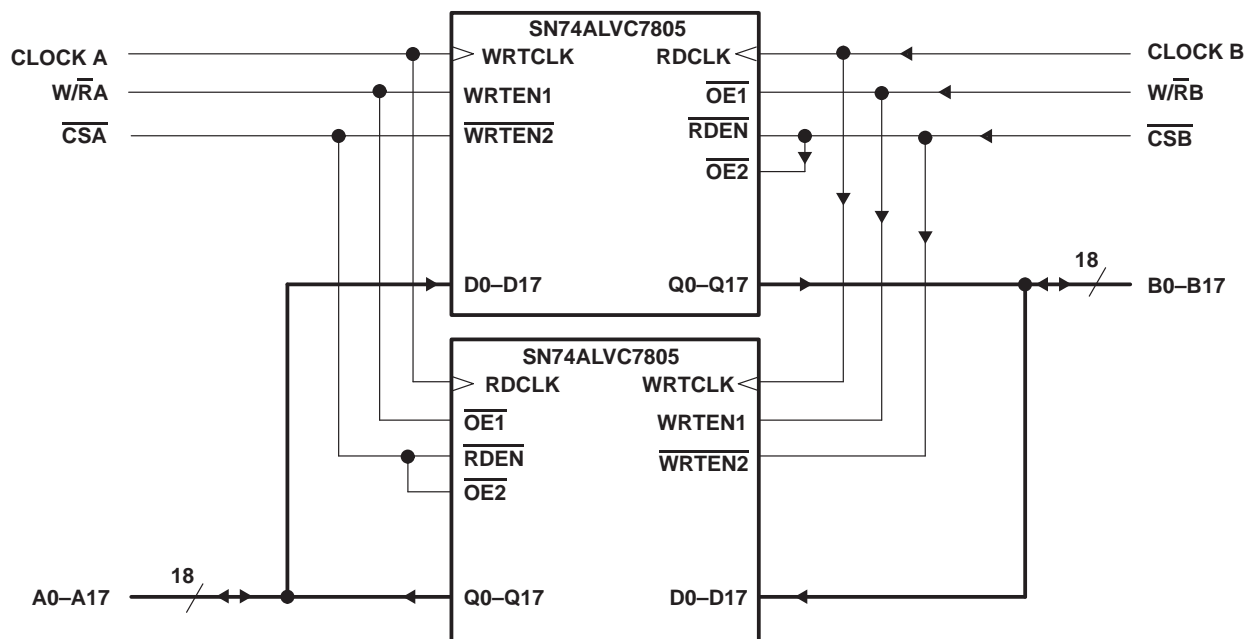
Figure 7. Bidirectional Configuration
