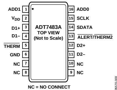
Figure 3.16-Lead QSOFP Pin Configuration
