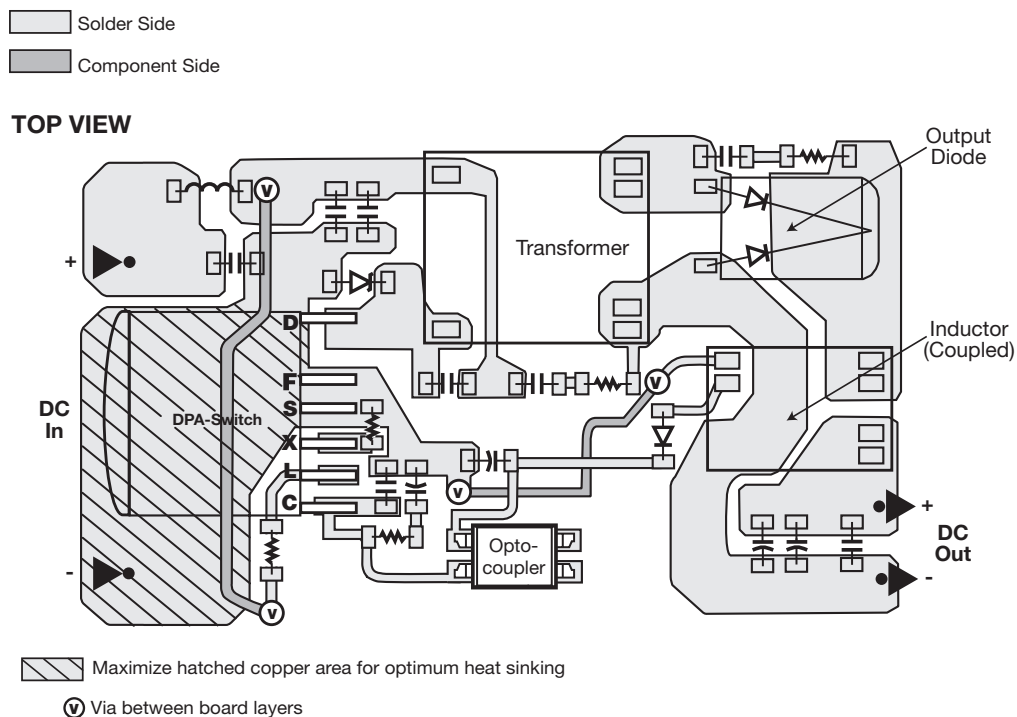
Figure 28. Layout Considerations for DPA-Switch Using R Package.
