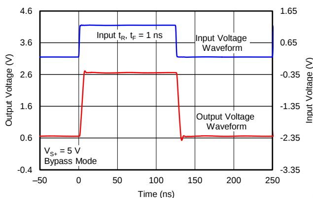
Figure 104. HD BYPASS LARGE-SIGNAL PULSE RESPONSE vs TIME
