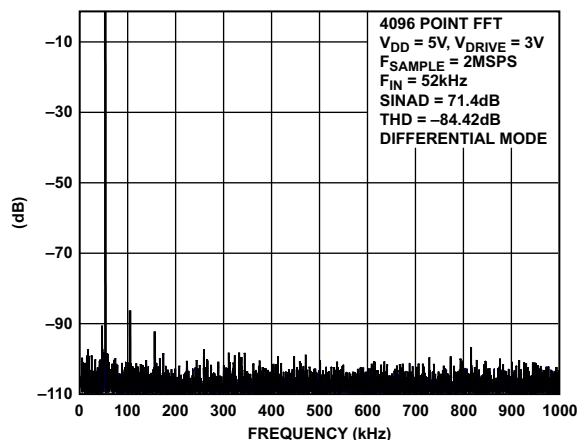
Figure 59. FFT
