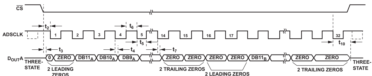
Figure 94. Reading Data from Both ADCs on One D_{\text{OUT}} Line with 32 ADSCLKs
