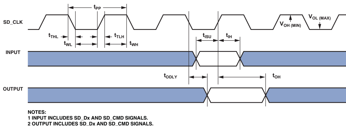
Figure 17. RSI Controller Timing (High-Speed Mode)
