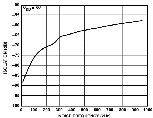
Figure 57. Channel-to-Channel Isolation
