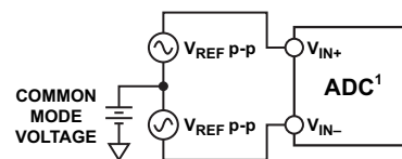
Figure 75. Differential Input Definition
