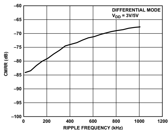
Figure 67. CMRR vs. Common-Mode Ripple Frequency
