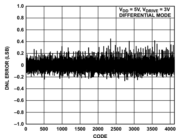
Figure 60. Typical DNL
