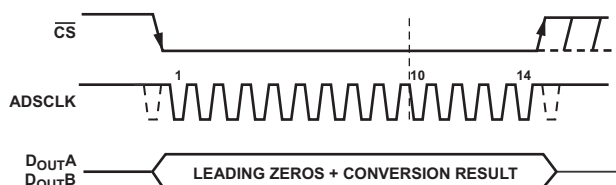
Figure 86. Normal Mode Operation
