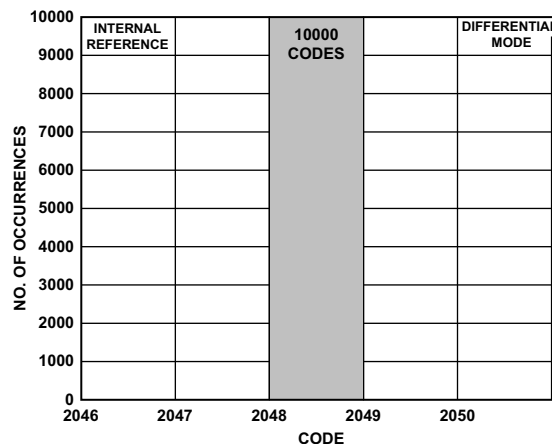
Figure 65. Histogram of Codes for 10k Samples in Differential Mode
