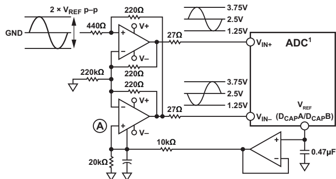
Figure 79. Dual Op Amp Circuit to Convert a Single-Ended Bipolar Signal into a Differential Unipolar Signal
