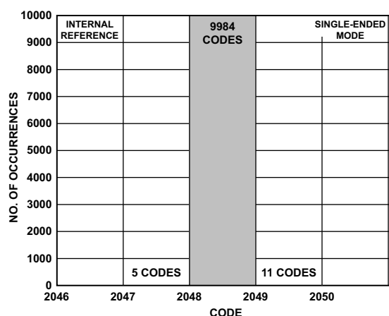
Figure 66. Histogram of Codes for 10k Samples in Single-Ended Mode
