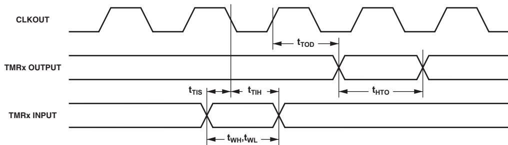
Figure 24. Timer Cycle Timing
