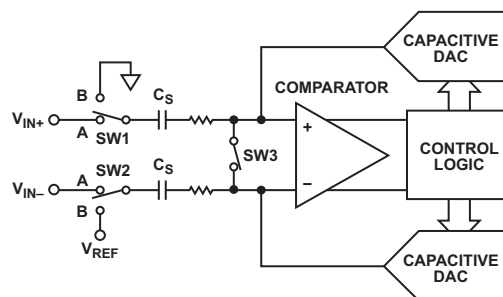
Figure 68. ADC Acquisition Phase
