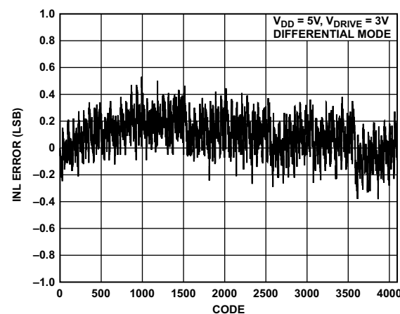
Figure 61. Typical INL
