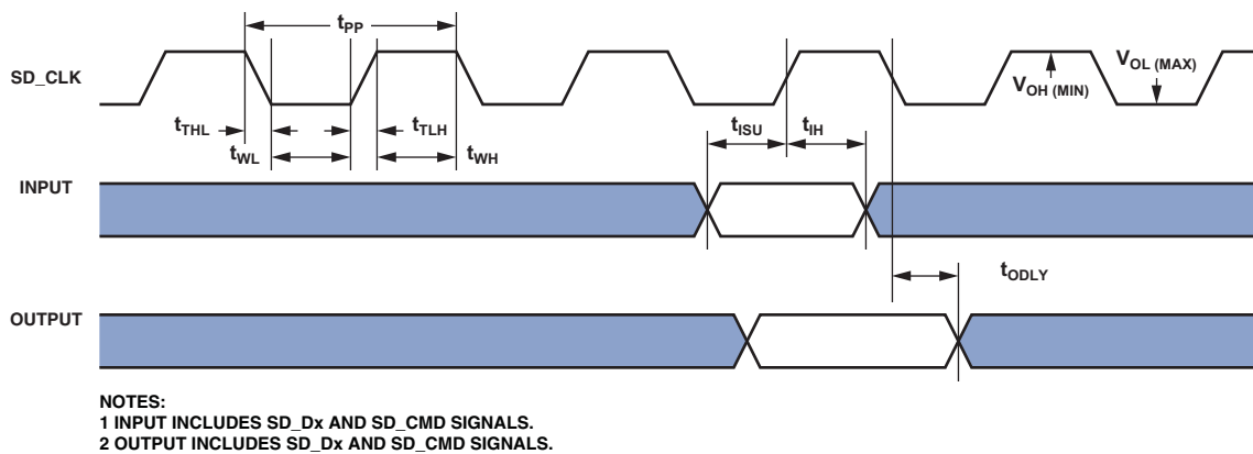
Figure 16. RSI Controller Timing
