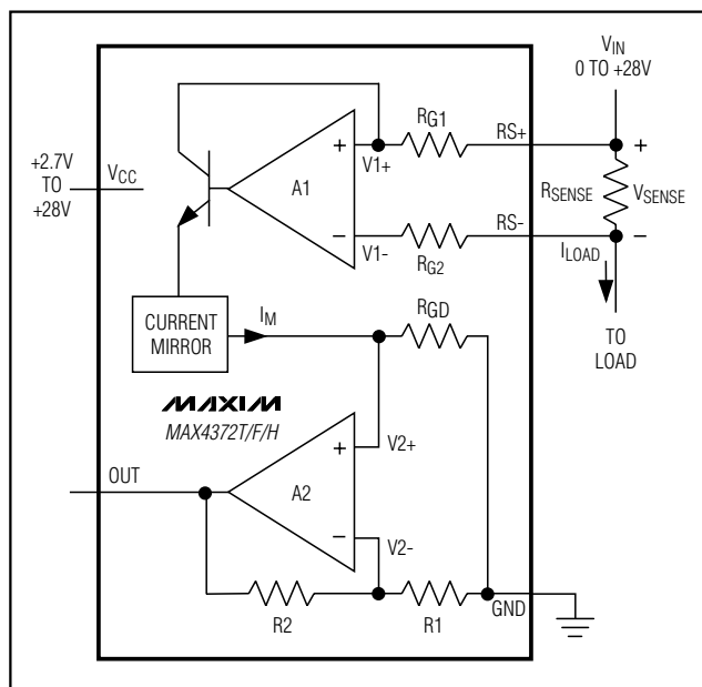
Figure 1. Functional Diagram
