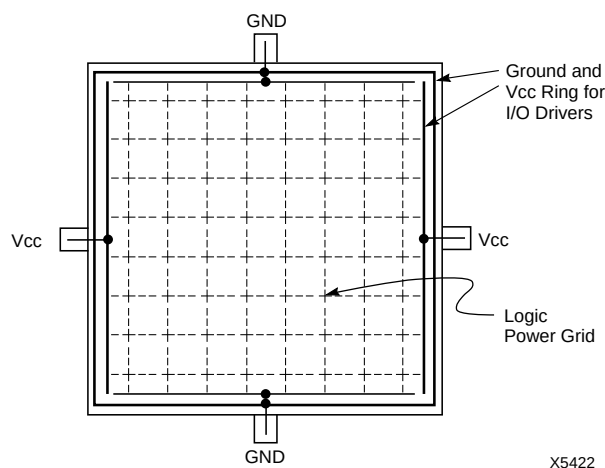
Figure 21: XC5200-Series Power Distribution
