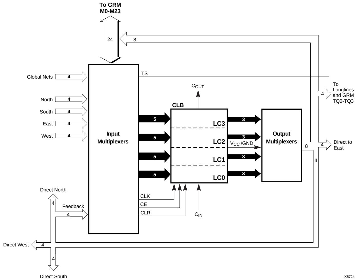
Figure 14: VersaBlock Details
